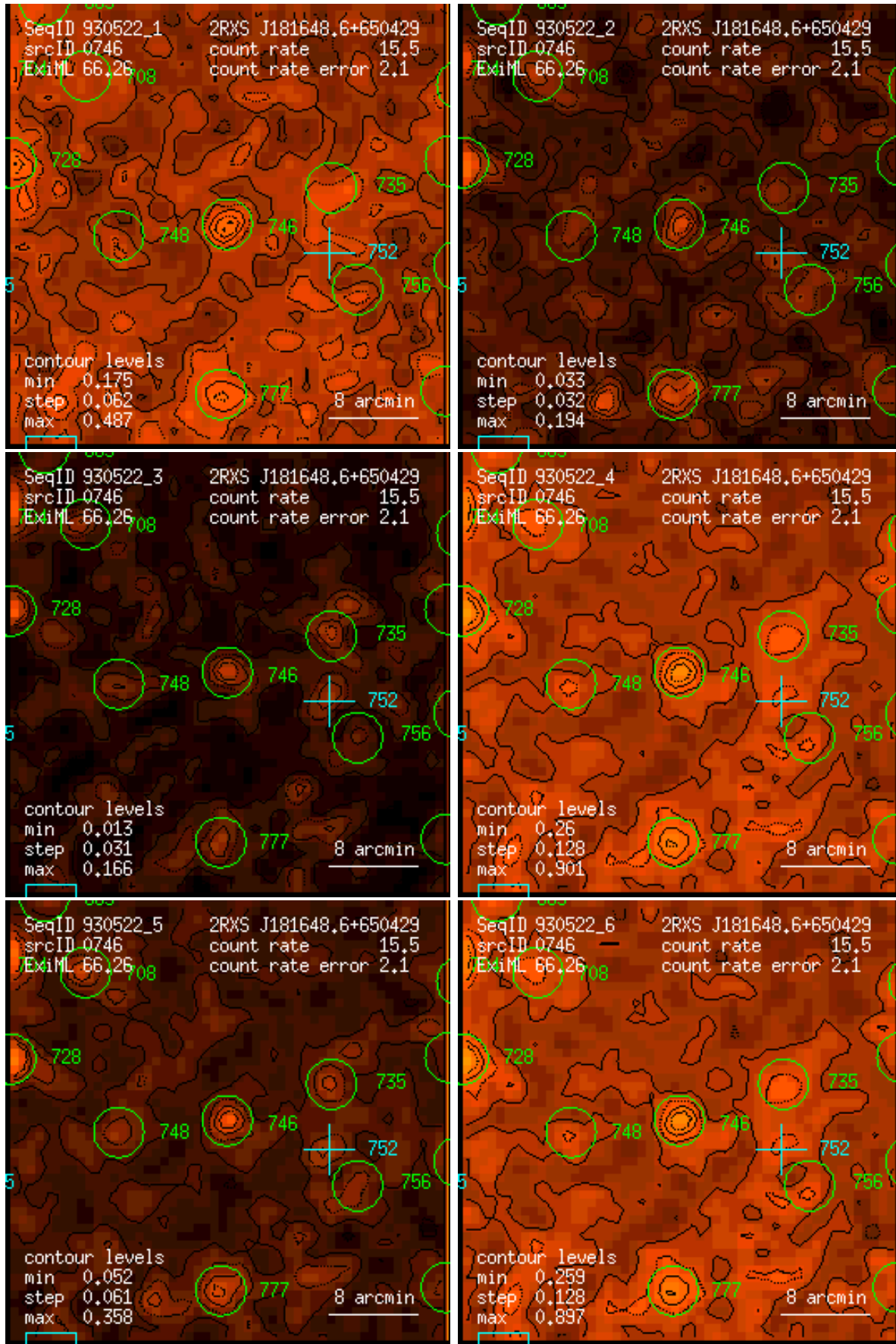
Figure 746: RASS 930522: detection 0746: band rate images, Gaussian filter: (1) PSPC channels 11 – 41, (2) 52 – 90, (3) 91 – 201, (4) 11 – 235, (5) 52 – 201, (6) 11 – 201. Broad band rates in counts/ks. Band rate contour levels in counts/ks/arcmin 2 .
