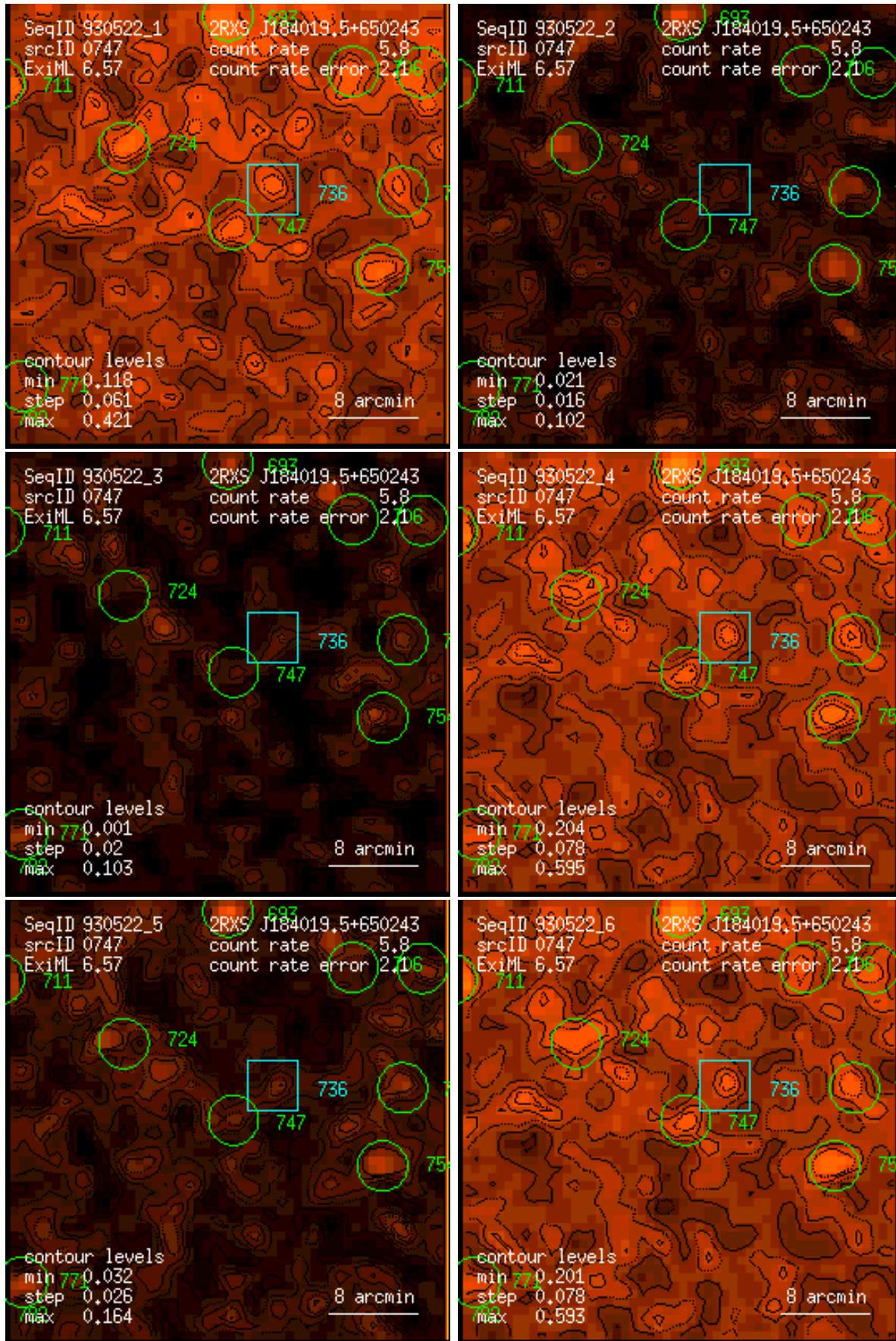
Figure 747: RASS 930522: detection 0747: band rate images, Gaussian filter: (1) PSPC channels 11 – 41, (2) 52 – 90, (3) 91 – 201, (4) 11 – 235, (5) 52 – 201, (6) 11 – 201. Broad band rates in counts/ks. Band rate contour levels in counts/ks/arcmin 2 .
