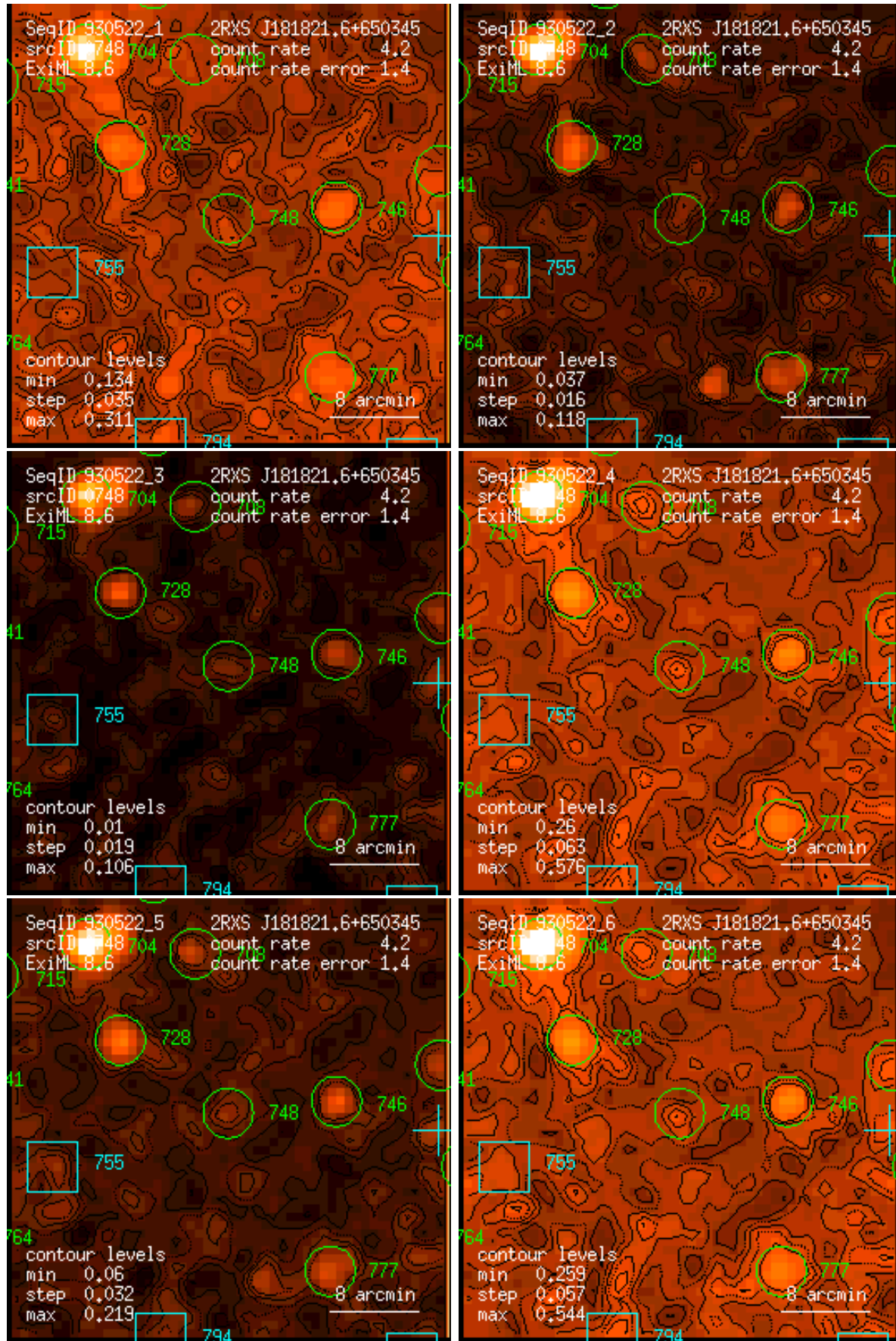
Figure 748: RASS 930522: detection 0748: band rate images, Gaussian filter: (1) PSPC channels 11 – 41, (2) 52 – 90, (3) 91 – 201, (4) 11 – 235, (5) 52 – 201, (6) 11 – 201. Broad band rates in counts/ks. Band rate contour levels in counts/ks/arcmin 2 .
