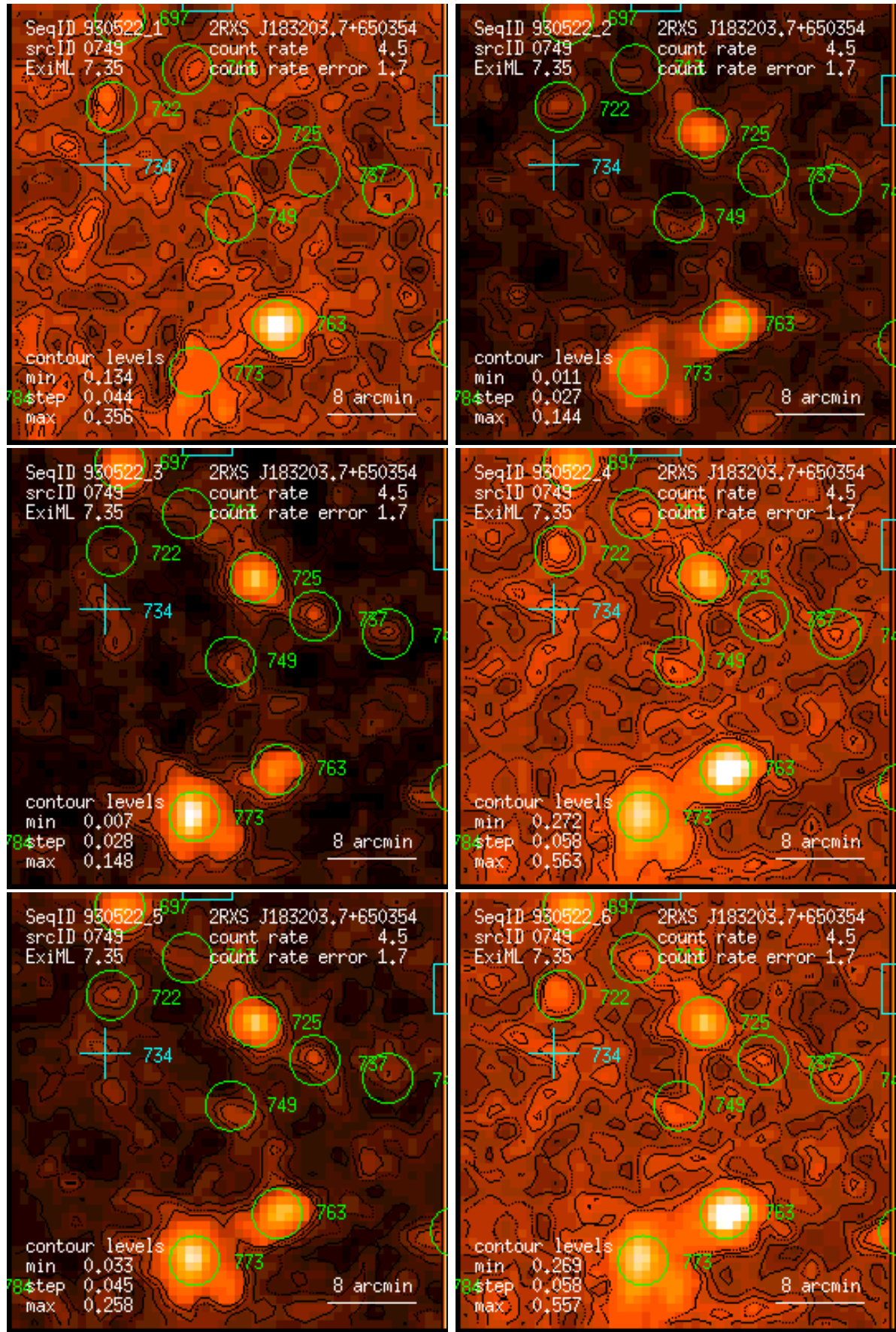
Figure 749: RASS 930522: detection 0749: band rate images, Gaussian filter: (1) PSPC channels 11 – 41, (2) 52 – 90, (3) 91 – 201, (4) 11 – 235, (5) 52 – 201, (6) 11 – 201. Broad band rates in counts/ks. Band rate contour levels in counts/ks/arcmin 2 .
