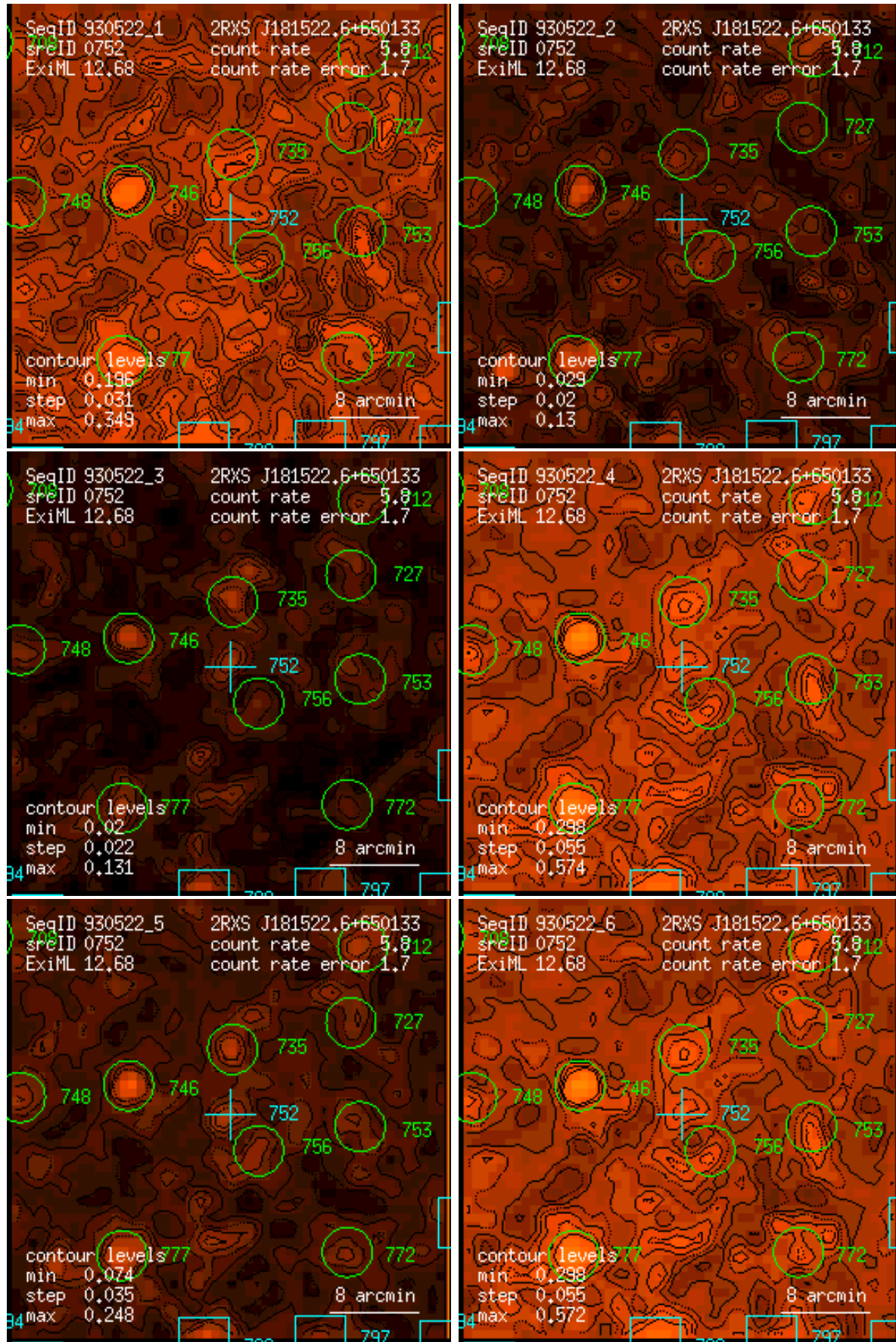
Figure 752: RASS 930522: detection 0752: band rate images, Gaussian filter: (1) PSPC channels 11 – 41, (2) 52 – 90, (3) 91 – 201, (4) 11 – 235, (5) 52 – 201, (6) 11 – 201. Broad band rates in counts/ks. Band rate contour levels in counts/ks/arcmin 2 .
