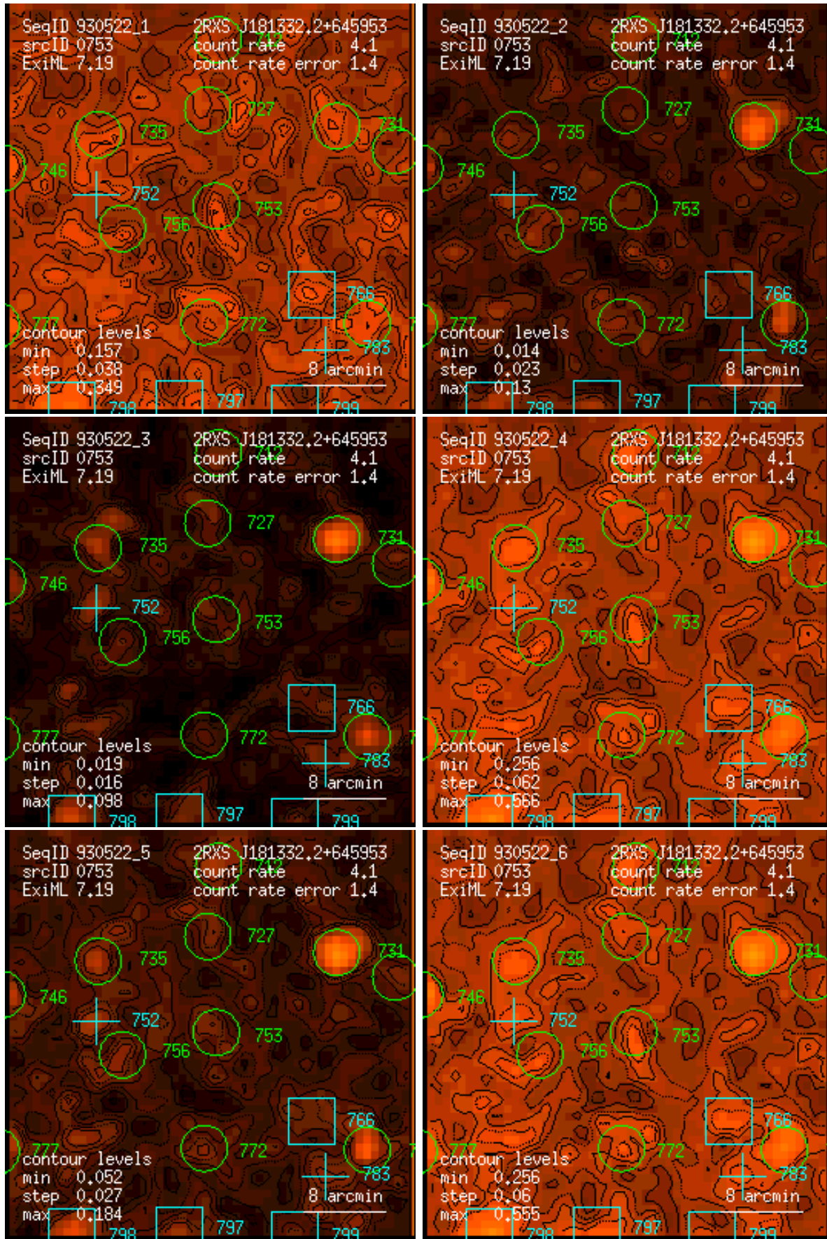
Figure 753: RASS 930522: detection 0753: band rate images, Gaussian filter: (1) PSPC channels 11 – 41, (2) 52 – 90, (3) 91 – 201, (4) 11 – 235, (5) 52 – 201, (6) 11 – 201. Broad band rates in counts/ks. Band rate contour levels in counts/ks/arcmin 2 .
