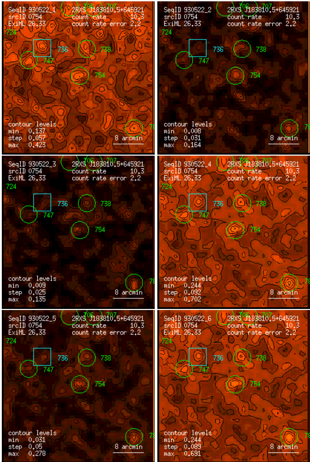
Figure 754: RASS 930522: detection 0754: band rate images, Gaussian filter: (1) PSPC channels 11 – 41, (2) 52 – 90, (3) 91 – 201, (4) 11 – 235, (5) 52 – 201, (6) 11 – 201. Broad band rates in counts/ks. Band rate contour levels in counts/ks/arcmin 2 .
