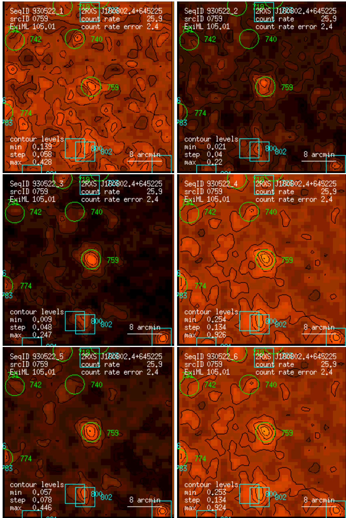
Figure 759: RASS 930522: detection 0759: band rate images, Gaussian filter: (1) PSPC channels 11 – 41, (2) 52 – 90, (3) 91 – 201, (4) 11 – 235, (5) 52 – 201, (6) 11 – 201. Broad band rates in counts/ks. Band rate contour levels in counts/ks/arcmin 2 .
