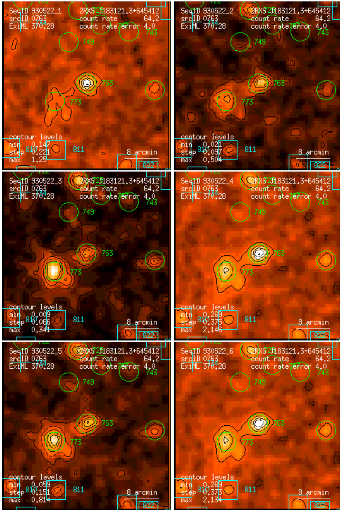
Figure 763: RASS 930522: detection 0763: band rate images, Gaussian filter: (1) PSPC channels 11 – 41, (2) 52 – 90, (3) 91 – 201, (4) 11 – 235, (5) 52 – 201, (6) 11 – 201. Broad band rates in counts/ks. Band rate contour levels in counts/ks/arcmin 2 .
