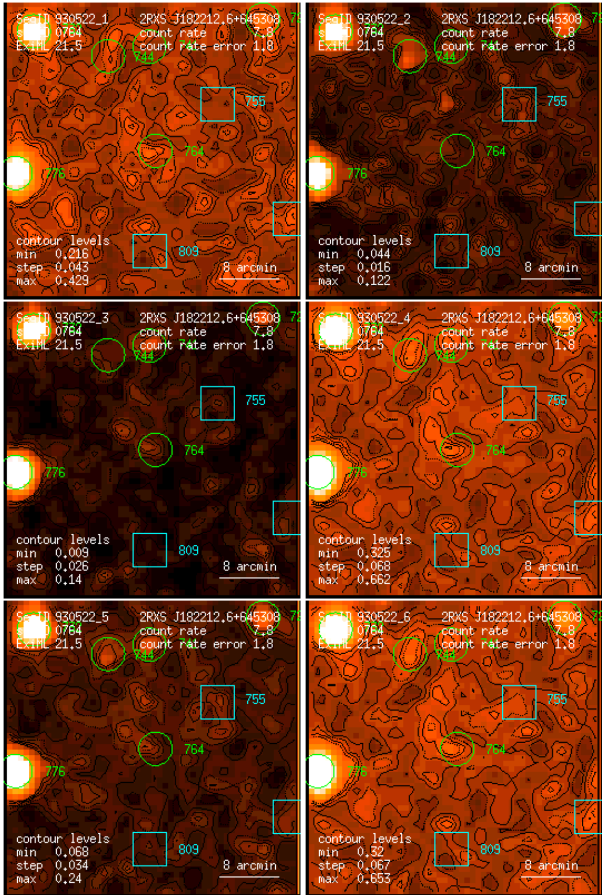
Figure 764: RASS 930522: detection 0764: band rate images, Gaussian filter: (1) PSPC channels 11 – 41, (2) 52 – 90, (3) 91 – 201, (4) 11 – 235, (5) 52 – 201, (6) 11 – 201. Broad band rates in counts/ks. Band rate contour levels in counts/ks/arcmin 2 .
