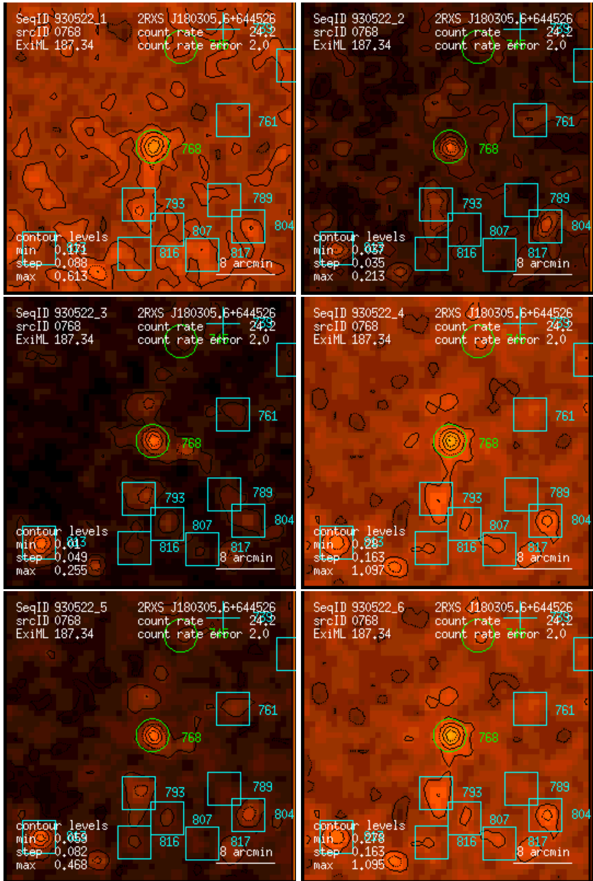
Figure 768: RASS 930522: detection 0768: band rate images, Gaussian filter: (1) PSPC channels 11 – 41, (2) 52 – 90, (3) 91 – 201, (4) 11 – 235, (5) 52 – 201, (6) 11 – 201. Broad band rates in counts/ks. Band rate contour levels in counts/ks/arcmin 2 .
