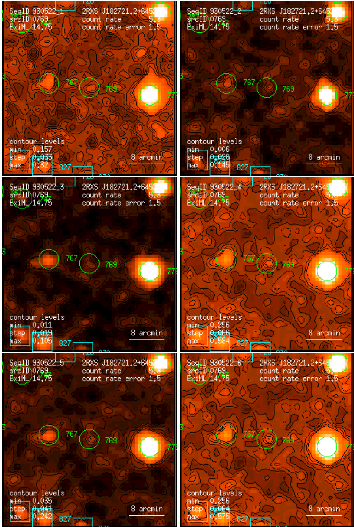
Figure 769: RASS 930522: detection 0769: band rate images, Gaussian filter: (1) PSPC channels 11 – 41, (2) 52 – 90, (3) 91 – 201, (4) 11 – 235, (5) 52 – 201, (6) 11 – 201. Broad band rates in counts/ks. Band rate contour levels in counts/ks/arcmin 2 .
