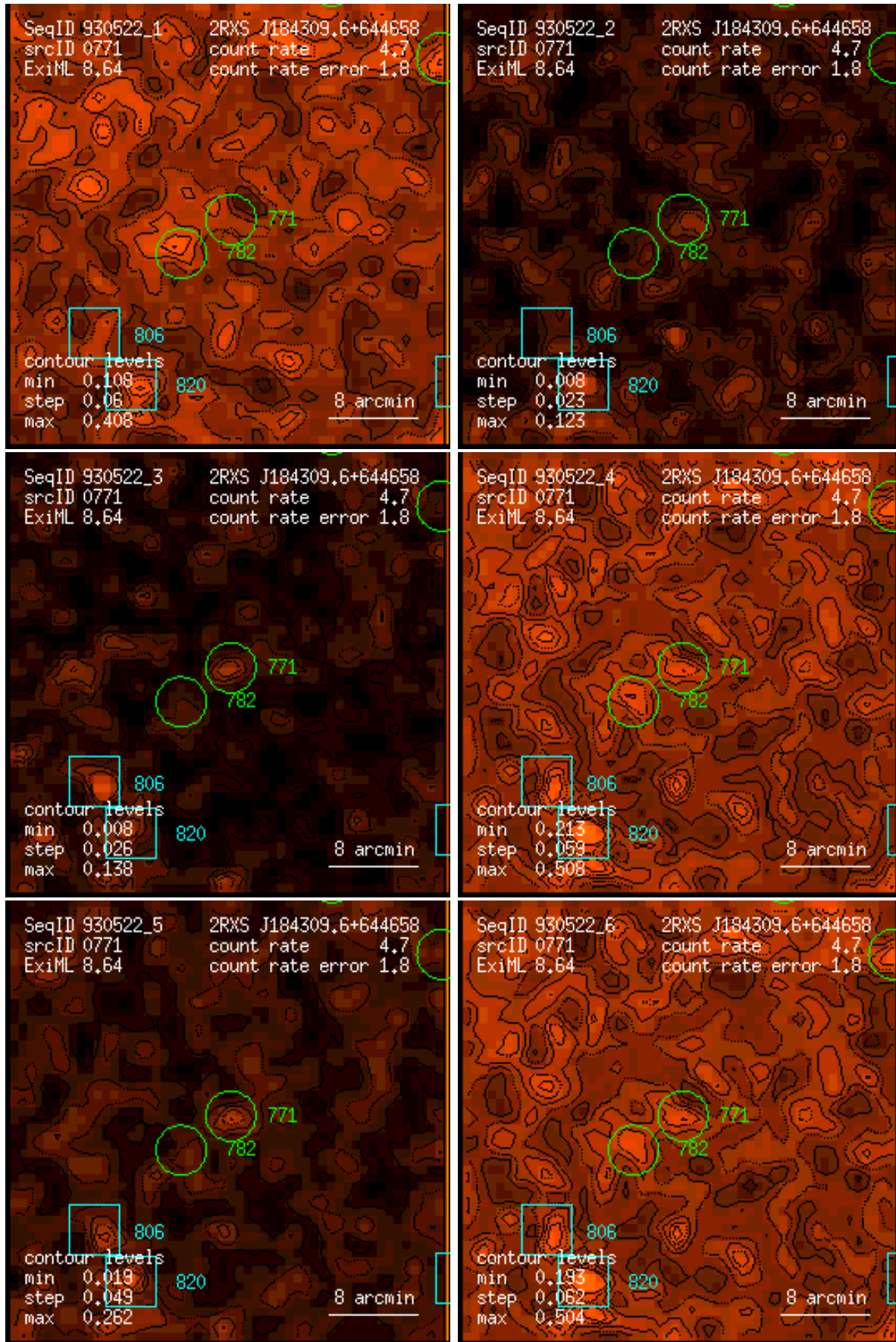
Figure 771: RASS 930522: detection 0771: band rate images, Gaussian filter: (1) PSPC channels 11 – 41, (2) 52 – 90, (3) 91 – 201, (4) 11 – 235, (5) 52 – 201, (6) 11 – 201. Broad band rates in counts/ks. Band rate contour levels in counts/ks/arcmin 2 .
