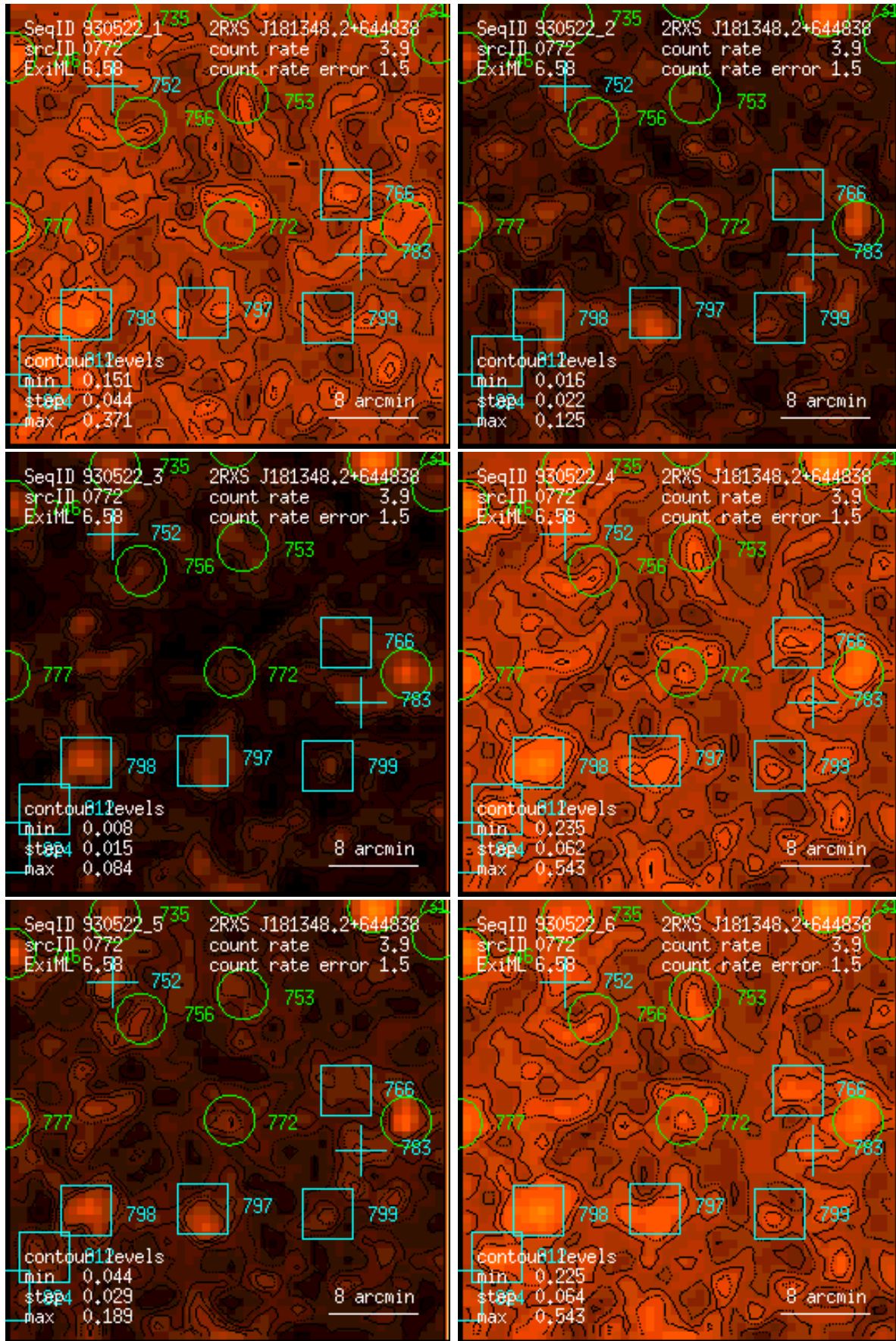
Figure 772: RASS 930522: detection 0772: band rate images, Gaussian filter: (1) PSPC channels 11 – 41, (2) 52 – 90, (3) 91 – 201, (4) 11 – 235, (5) 52 – 201, (6) 11 – 201. Broad band rates in counts/ks. Band rate contour levels in counts/ks/arcmin 2 .
