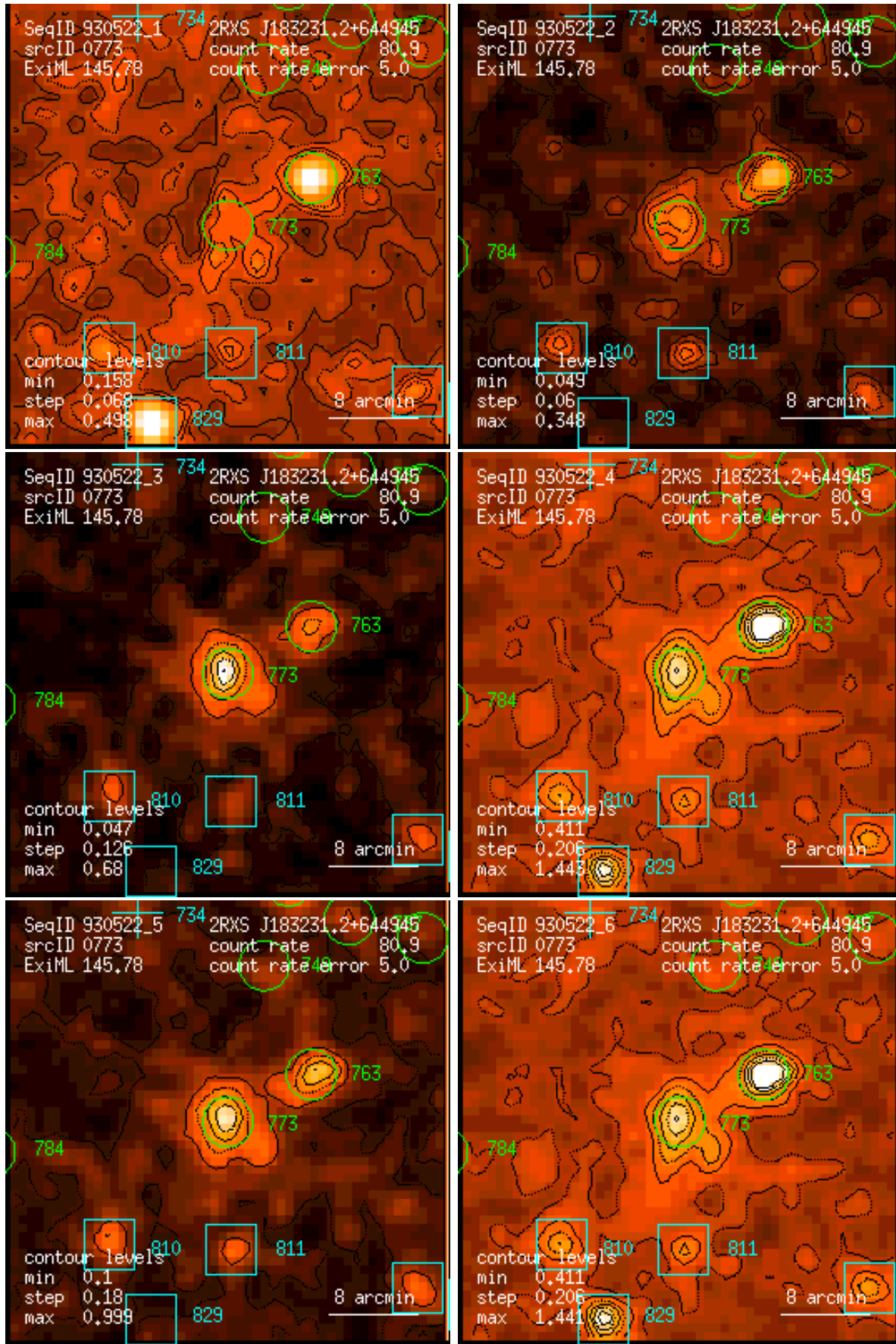
Figure 773: RASS 930522: detection 0773: band rate images, Gaussian filter: (1) PSPC channels 11 – 41, (2) 52 – 90, (3) 91 – 201, (4) 11 – 235, (5) 52 – 201, (6) 11 – 201. Broad band rates in counts/ks. Band rate contour levels in counts/ks/arcmin 2 .
