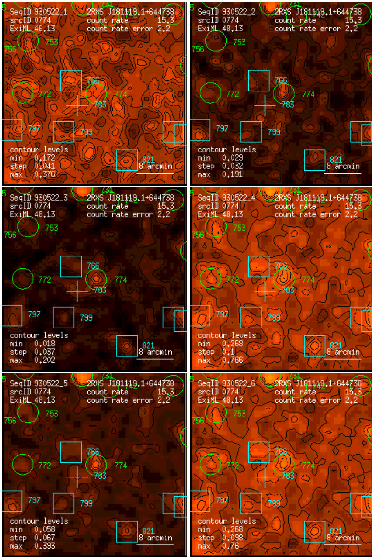
Figure 774: RASS 930522: detection 0774: band rate images, Gaussian filter: (1) PSPC channels 11 – 41, (2) 52 – 90, (3) 91 – 201, (4) 11 – 235, (5) 52 – 201, (6) 11 – 201. Broad band rates in counts/ks. Band rate contour levels in counts/ks/arcmin 2 .
