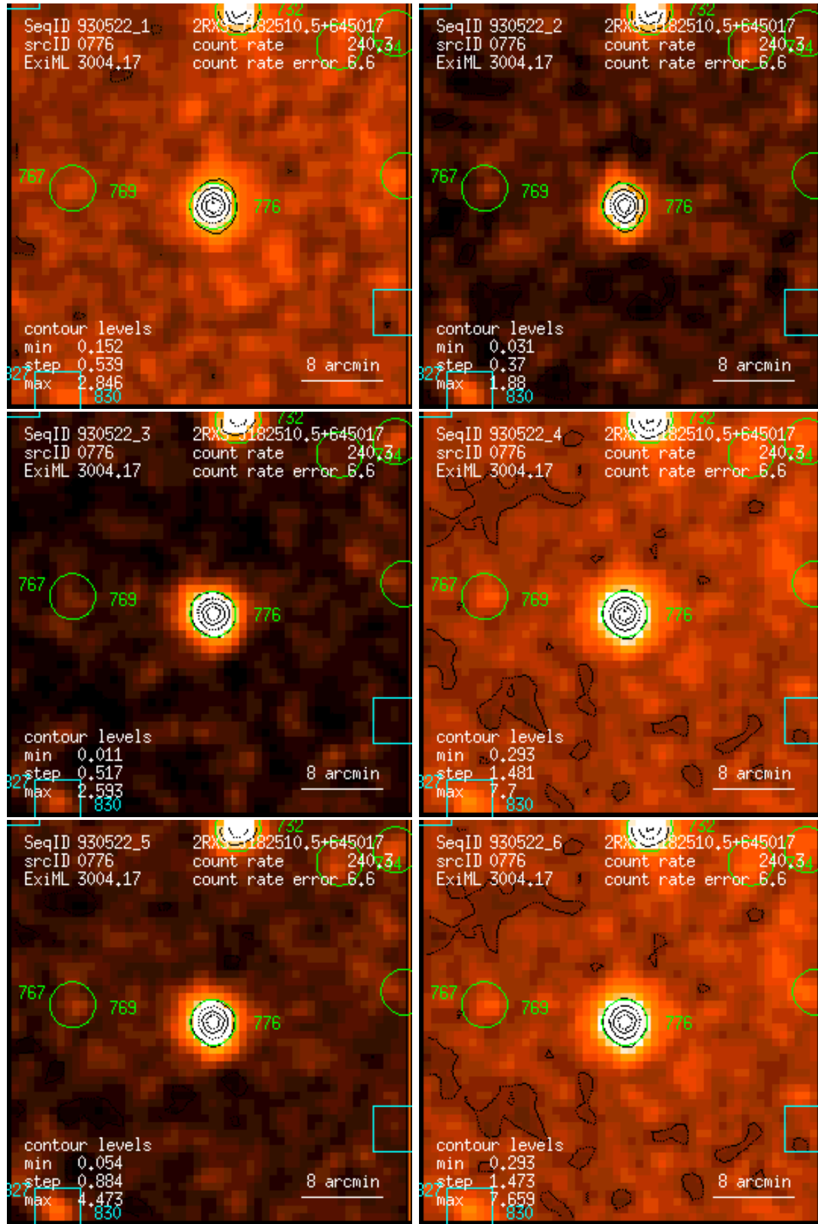
Figure 776: RASS 930522: detection 0776: band rate images, Gaussian filter: (1) PSPC channels 11 – 41, (2) 52 – 90, (3) 91 – 201, (4) 11 – 235, (5) 52 – 201, (6) 11 – 201. Broad band rates in counts/ks. Band rate contour levels in counts/ks/arcmin 2 .
