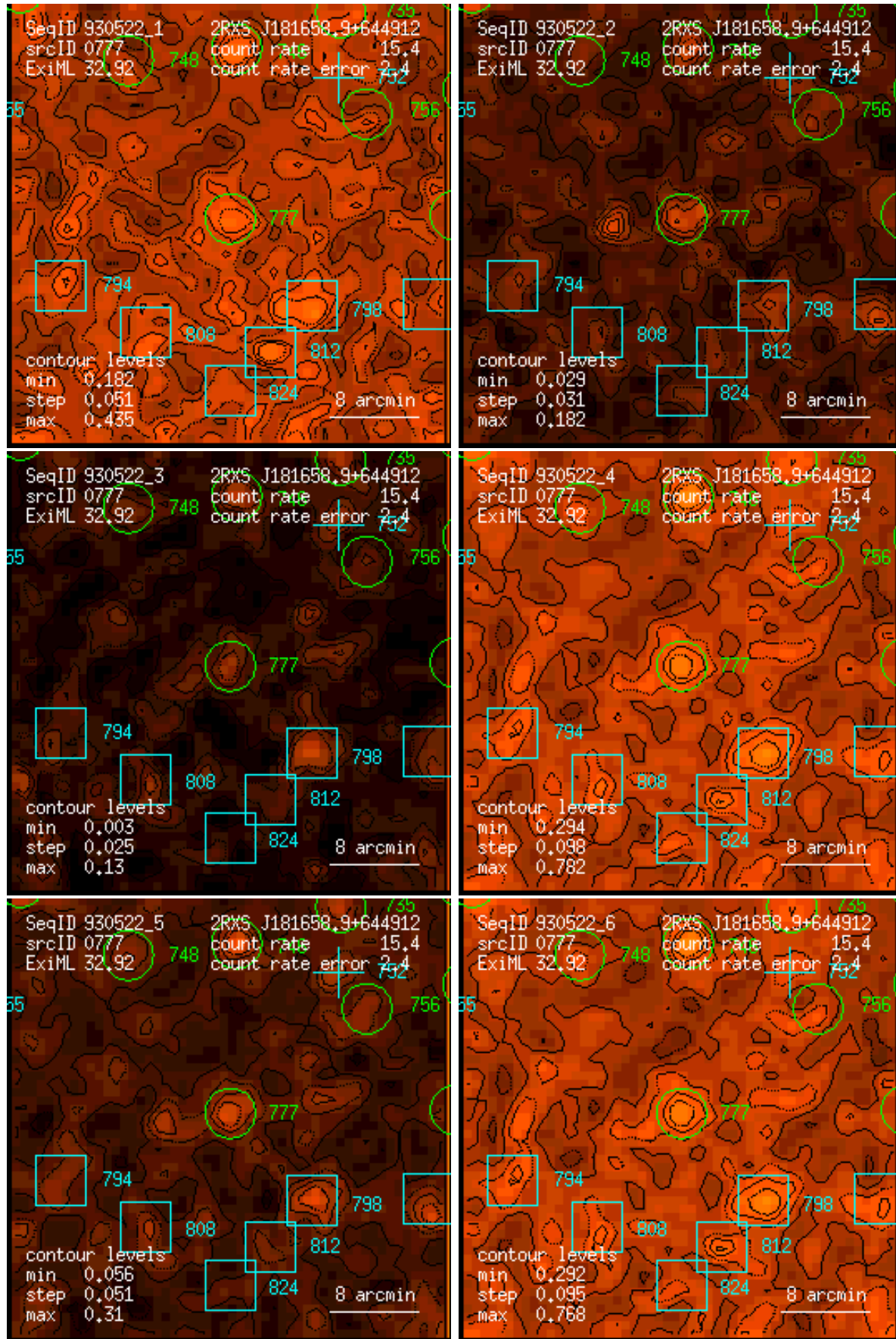
Figure 777: RASS 930522: detection 0777: band rate images, Gaussian filter: (1) PSPC channels 11 – 41, (2) 52 – 90, (3) 91 – 201, (4) 11 – 235, (5) 52 – 201, (6) 11 – 201. Broad band rates in counts/ks. Band rate contour levels in counts/ks/arcmin 2 .
