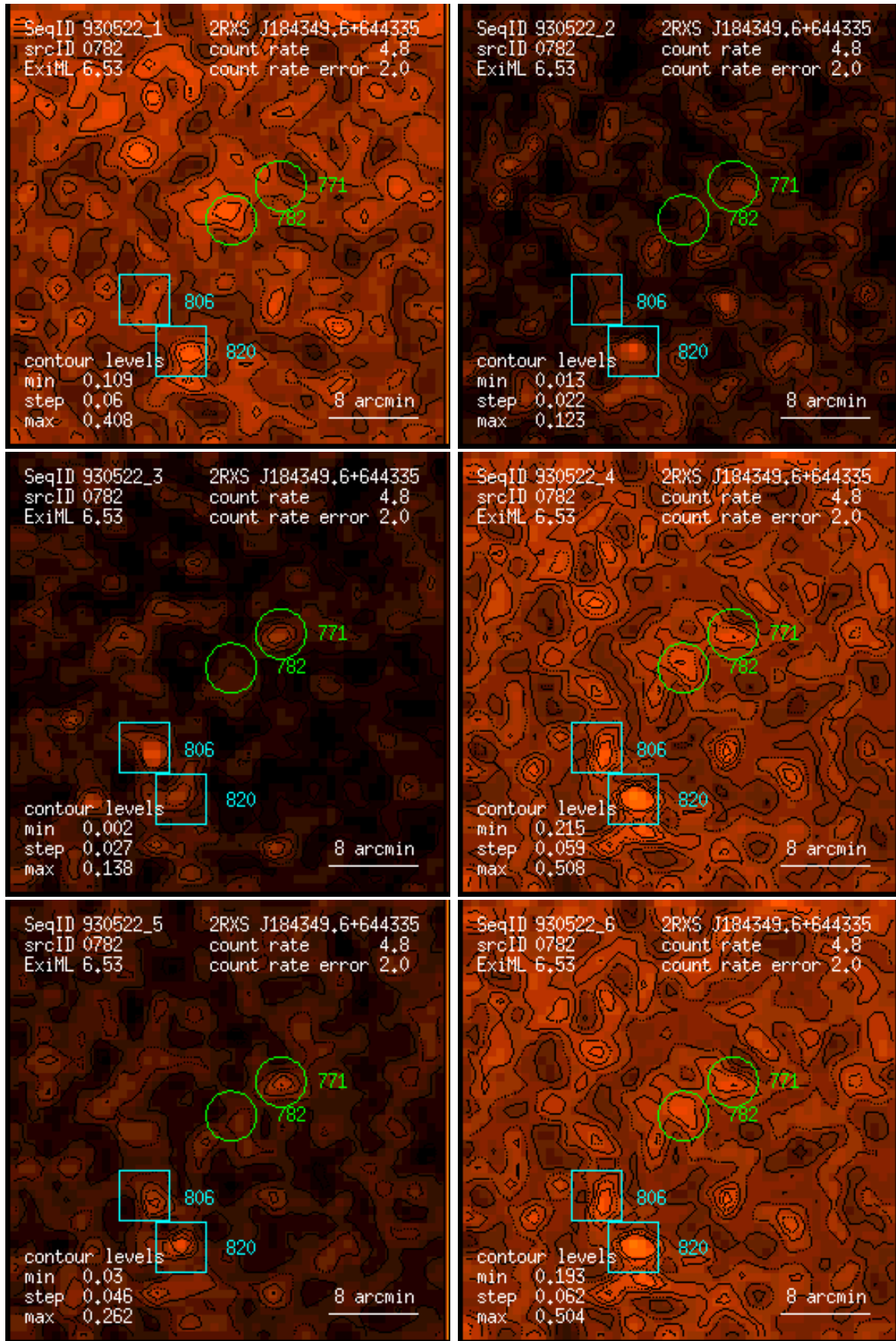
Figure 782: RASS 930522: detection 0782: band rate images, Gaussian filter: (1) PSPC channels 11 – 41, (2) 52 – 90, (3) 91 – 201, (4) 11 – 235, (5) 52 – 201, (6) 11 – 201. Broad band rates in counts/ks. Band rate contour levels in counts/ks/arcmin 2 .
