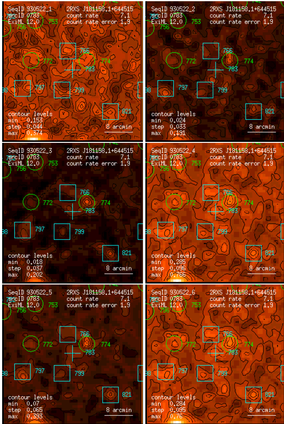
Figure 783: RASS 930522: detection 0783: band rate images, Gaussian filter: (1) PSPC channels 11 – 41, (2) 52 – 90, (3) 91 – 201, (4) 11 – 235, (5) 52 – 201, (6) 11 – 201. Broad band rates in counts/ks. Band rate contour levels in counts/ks/arcmin 2 .
