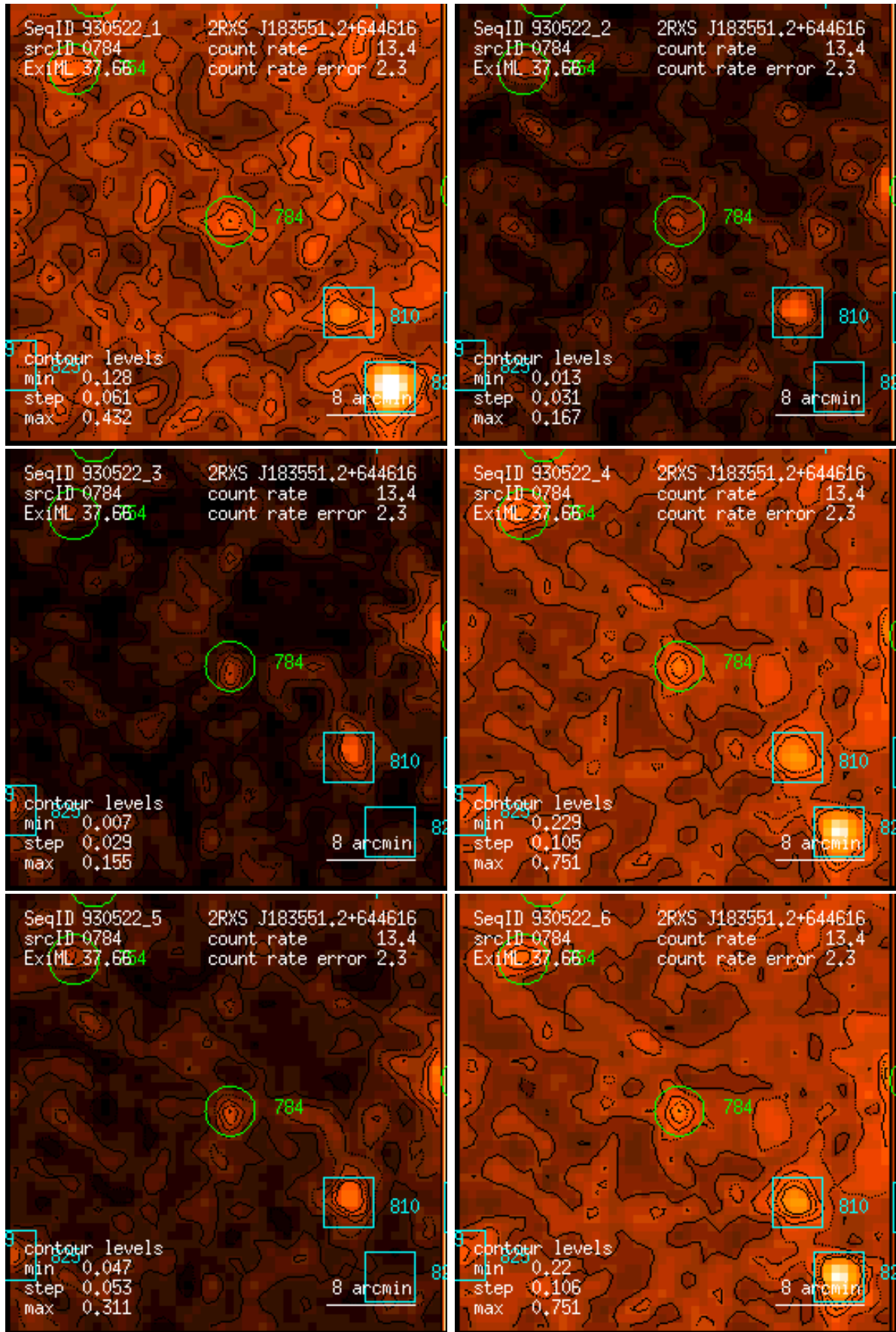
Figure 784: RASS 930522: detection 0784: band rate images, Gaussian filter: (1) PSPC channels 11 – 41, (2) 52 – 90, (3) 91 – 201, (4) 11 – 235, (5) 52 – 201, (6) 11 – 201. Broad band rates in counts/ks. Band rate contour levels in counts/ks/arcmin 2 .
