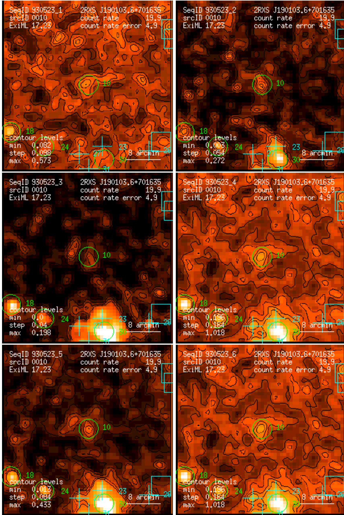
Figure 10: RASS 930523: detection 0010: band rate images, Gaussian filter: (1) PSPC channels 11 – 41, (2) 52 – 90, (3) 91 – 201, (4) 11 – 235, (5) 52 – 201, (6) 11 – 201. Broad band rates in counts/ks. Band rate contour levels in counts/ks/arcmin 2 .
