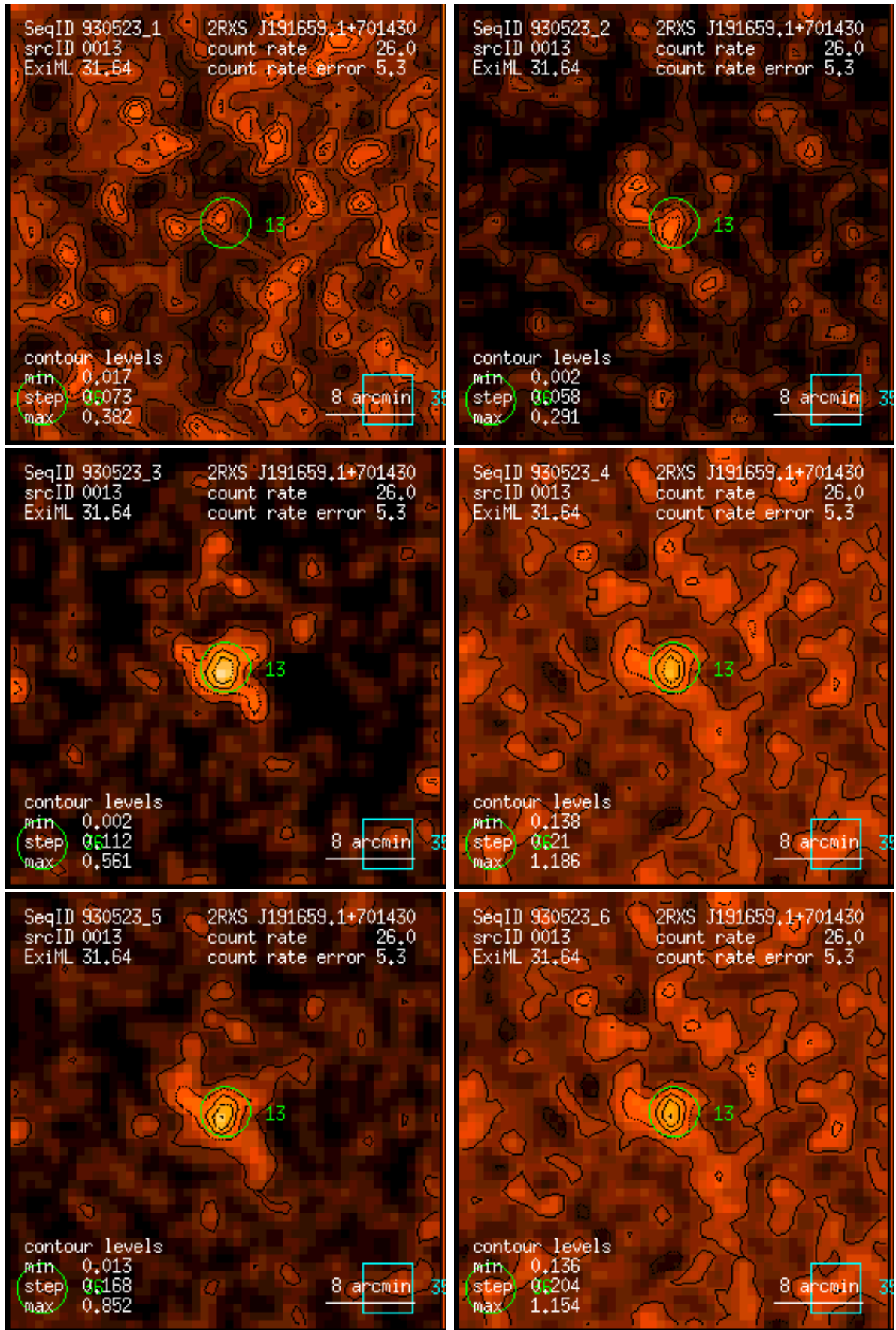
Figure 13: RASS 930523: detection 0013: band rate images, Gaussian filter: (1) PSPC channels 11 – 41, (2) 52 – 90, (3) 91 – 201, (4) 11 – 235, (5) 52 – 201, (6) 11 – 201. Broad band rates in counts/ks. Band rate contour levels in counts/ks/arcmin 2 .
