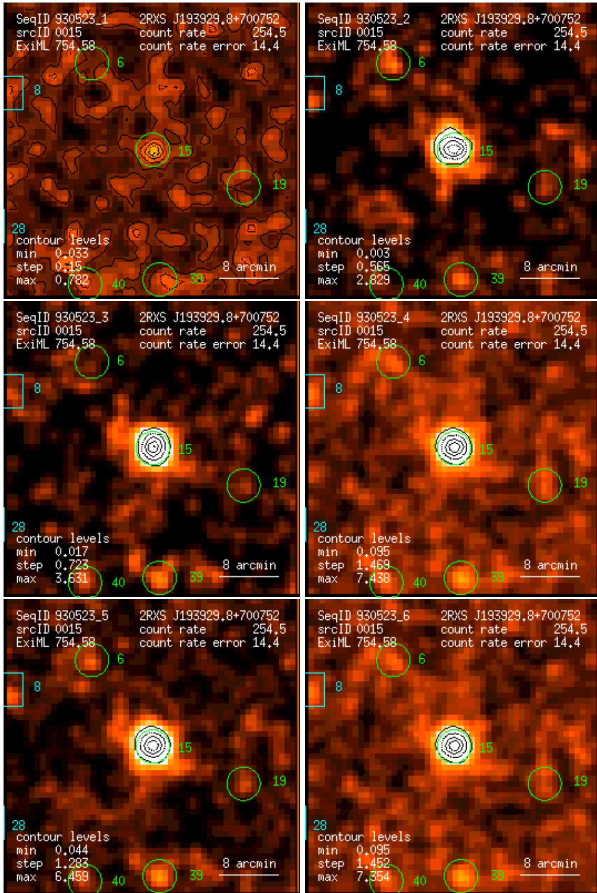
Figure 15: RASS 930523: detection 0015: band rate images, Gaussian filter: (1) PSPC channels 11 – 41, (2) 52 – 90, (3) 91 – 201, (4) 11 – 235, (5) 52 – 201, (6) 11 – 201. Broad band rates in counts/ks. Band rate contour levels in counts/ks/arcmin 2 .
