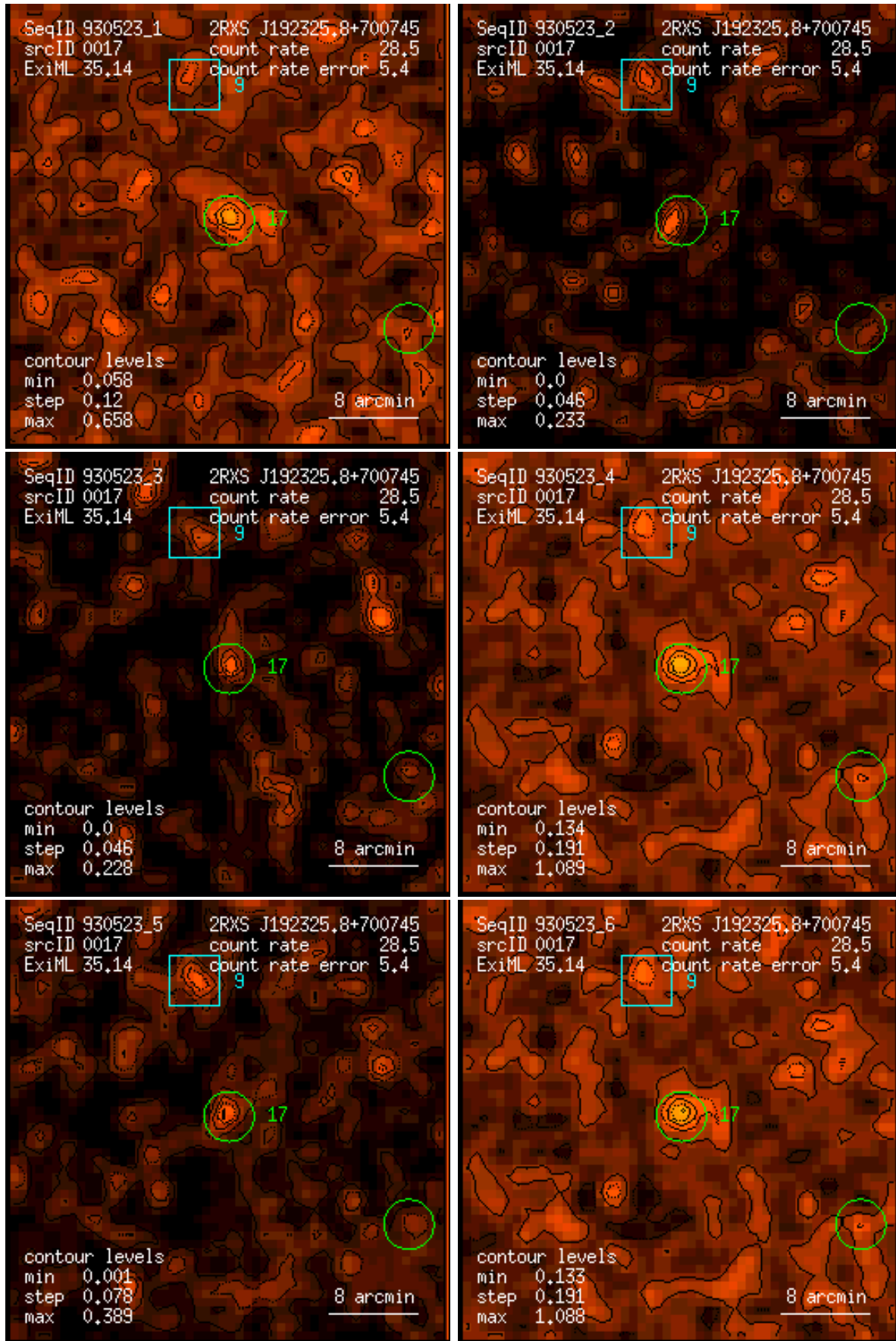
Figure 17: RASS 930523: detection 0017: band rate images, Gaussian filter: (1) PSPC channels 11 – 41, (2) 52 – 90, (3) 91 – 201, (4) 11 – 235, (5) 52 – 201, (6) 11 – 201. Broad band rates in counts/ks. Band rate contour levels in counts/ks/arcmin 2 .
