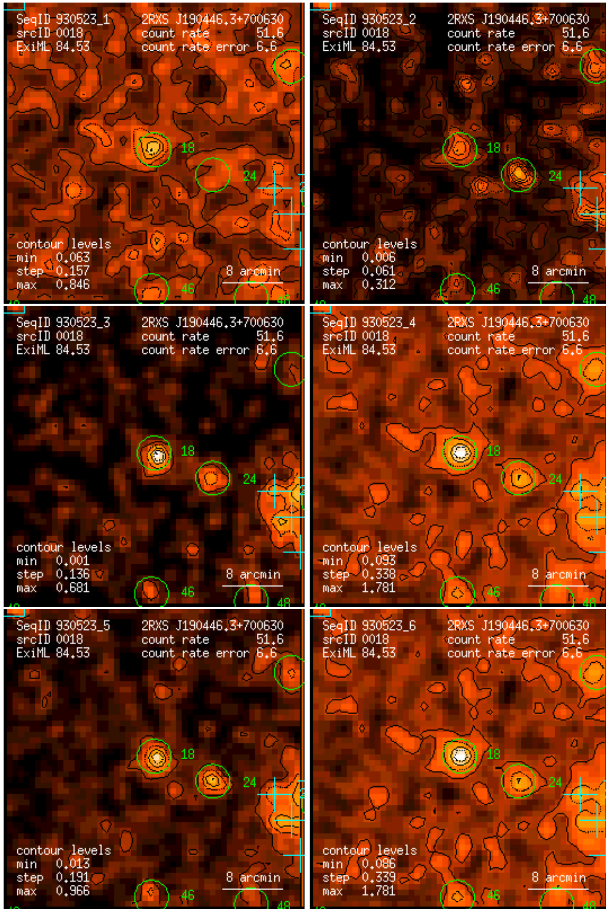
Figure 18: RASS 930523: detection 0018: band rate images, Gaussian filter: (1) PSPC channels 11 – 41, (2) 52 – 90, (3) 91 – 201, (4) 11 – 235, (5) 52 – 201, (6) 11 – 201. Broad band rates in counts/ks. Band rate contour levels in counts/ks/arcmin 2 .
