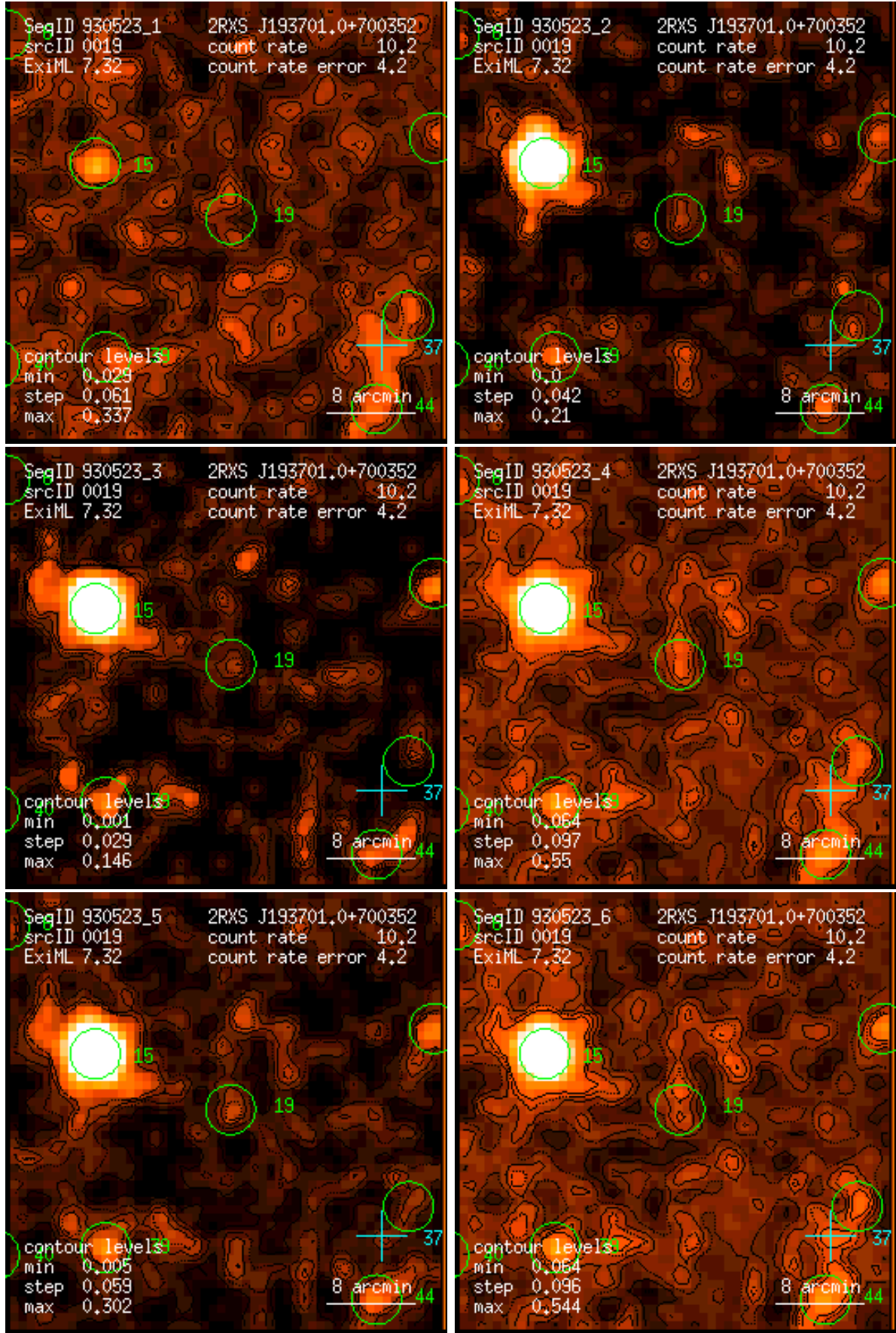
Figure 19: RASS 930523: detection 0019: band rate images, Gaussian filter: (1) PSPC channels 11 – 41, (2) 52 – 90, (3) 91 – 201, (4) 11 – 235, (5) 52 – 201, (6) 11 – 201. Broad band rates in counts/ks. Band rate contour levels in counts/ks/arcmin 2 .
