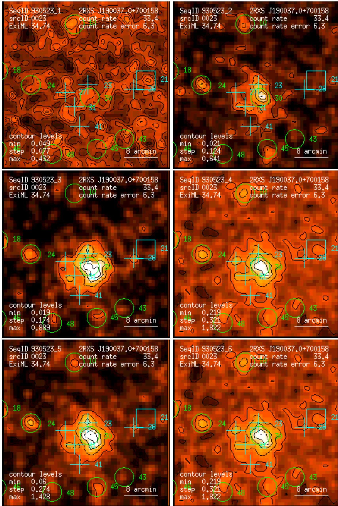
Figure 23: RASS 930523: detection 0023: band rate images, Gaussian filter: (1) PSPC channels 11 – 41, (2) 52 – 90, (3) 91 – 201, (4) 11 – 235, (5) 52 – 201, (6) 11 – 201. Broad band rates in counts/ks. Band rate contour levels in counts/ks/arcmin 2 .
