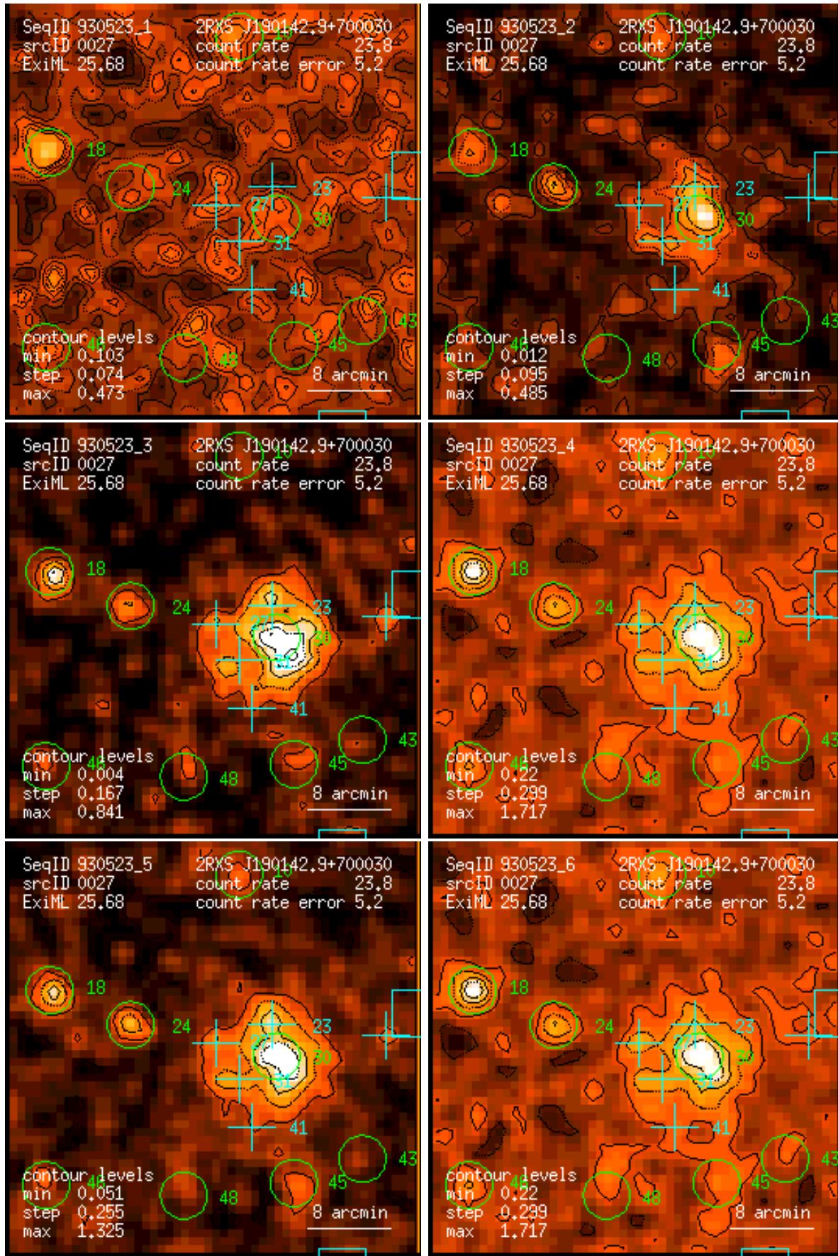
Figure 27: RASS 930523: detection 0027: band rate images, Gaussian filter: (1) PSPC channels 11 – 41, (2) 52 – 90, (3) 91 – 201, (4) 11 – 235, (5) 52 – 201, (6) 11 – 201. Broad band rates in counts/ks. Band rate contour levels in counts/ks/arcmin 2 .
