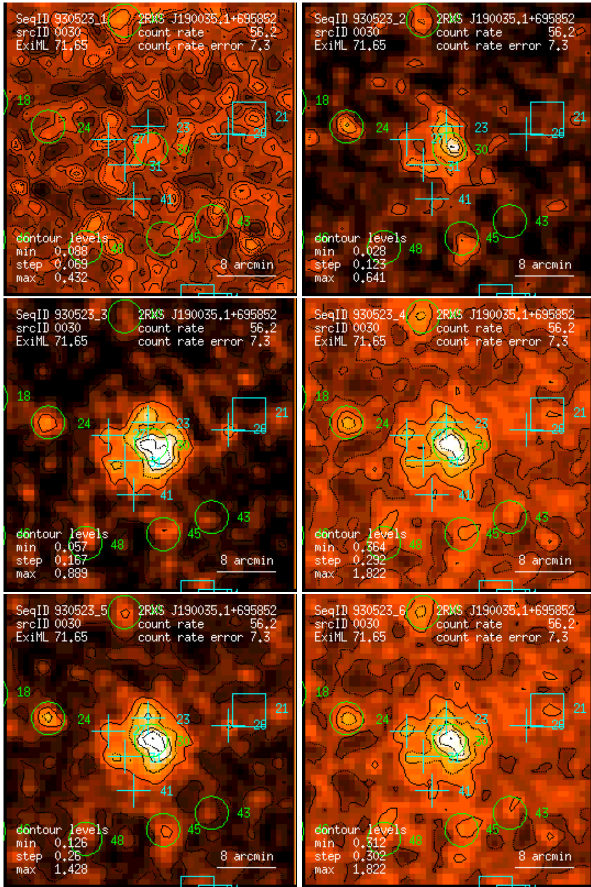
Figure 30: RASS 930523: detection 0030: band rate images, Gaussian filter: (1) PSPC channels 11 – 41, (2) 52 – 90, (3) 91 – 201, (4) 11 – 235, (5) 52 – 201, (6) 11 – 201. Broad band rates in counts/ks. Band rate contour levels in counts/ks/arcmin 2 .
