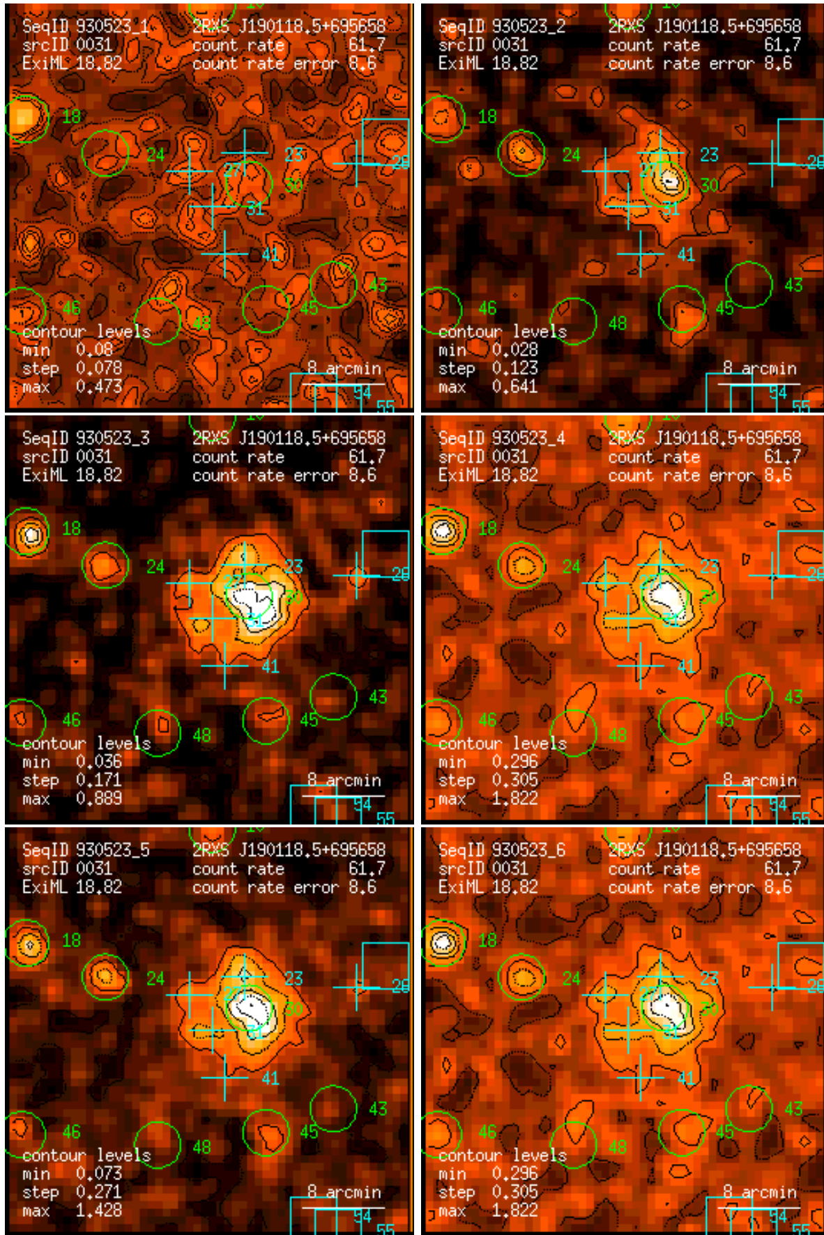
Figure 31: RASS 930523: detection 0031: band rate images, Gaussian filter: (1) PSPC channels 11 – 41, (2) 52 – 90, (3) 91 – 201, (4) 11 – 235, (5) 52 – 201, (6) 11 – 201. Broad band rates in counts/ks. Band rate contour levels in counts/ks/arcmin 2 .
