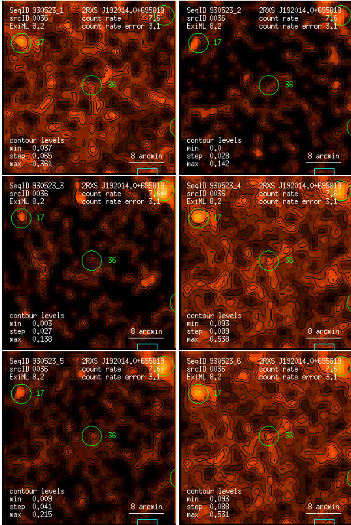
Figure 36: RASS 930523: detection 0036: band rate images, Gaussian filter: (1) PSPC channels 11 – 41, (2) 52 – 90, (3) 91 – 201, (4) 11 – 235, (5) 52 – 201, (6) 11 – 201. Broad band rates in counts/ks. Band rate contour levels in counts/ks/arcmin 2 .
