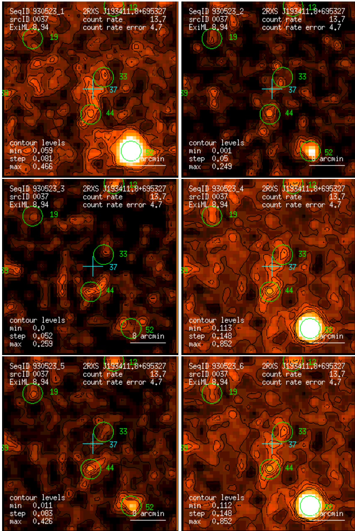
Figure 37: RASS 930523: detection 0037: band rate images, Gaussian filter: (1) PSPC channels 11 – 41, (2) 52 – 90, (3) 91 – 201, (4) 11 – 235, (5) 52 – 201, (6) 11 – 201. Broad band rates in counts/ks. Band rate contour levels in counts/ks/arcmin 2 .
