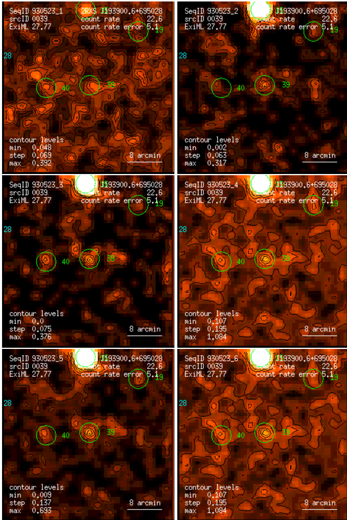
Figure 39: RASS 930523: detection 0039: band rate images, Gaussian filter: (1) PSPC channels 11 – 41, (2) 52 – 90, (3) 91 – 201, (4) 11 – 235, (5) 52 – 201, (6) 11 – 201. Broad band rates in counts/ks. Band rate contour levels in counts/ks/arcmin 2 .
