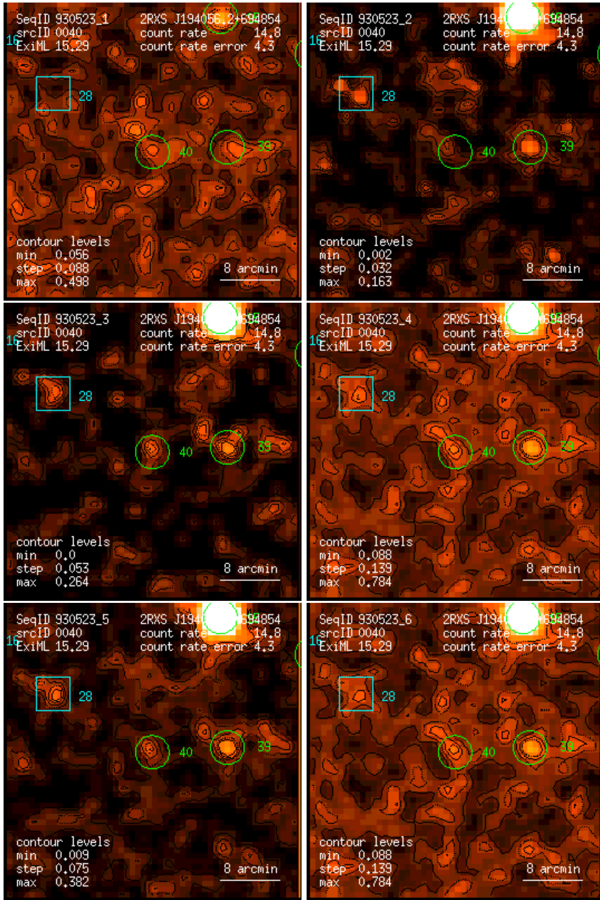
Figure 40: RASS 930523: detection 0040: band rate images, Gaussian filter: (1) PSPC channels 11 – 41, (2) 52 – 90, (3) 91 – 201, (4) 11 – 235, (5) 52 – 201, (6) 11 – 201. Broad band rates in counts/ks. Band rate contour levels in counts/ks/arcmin 2 .
