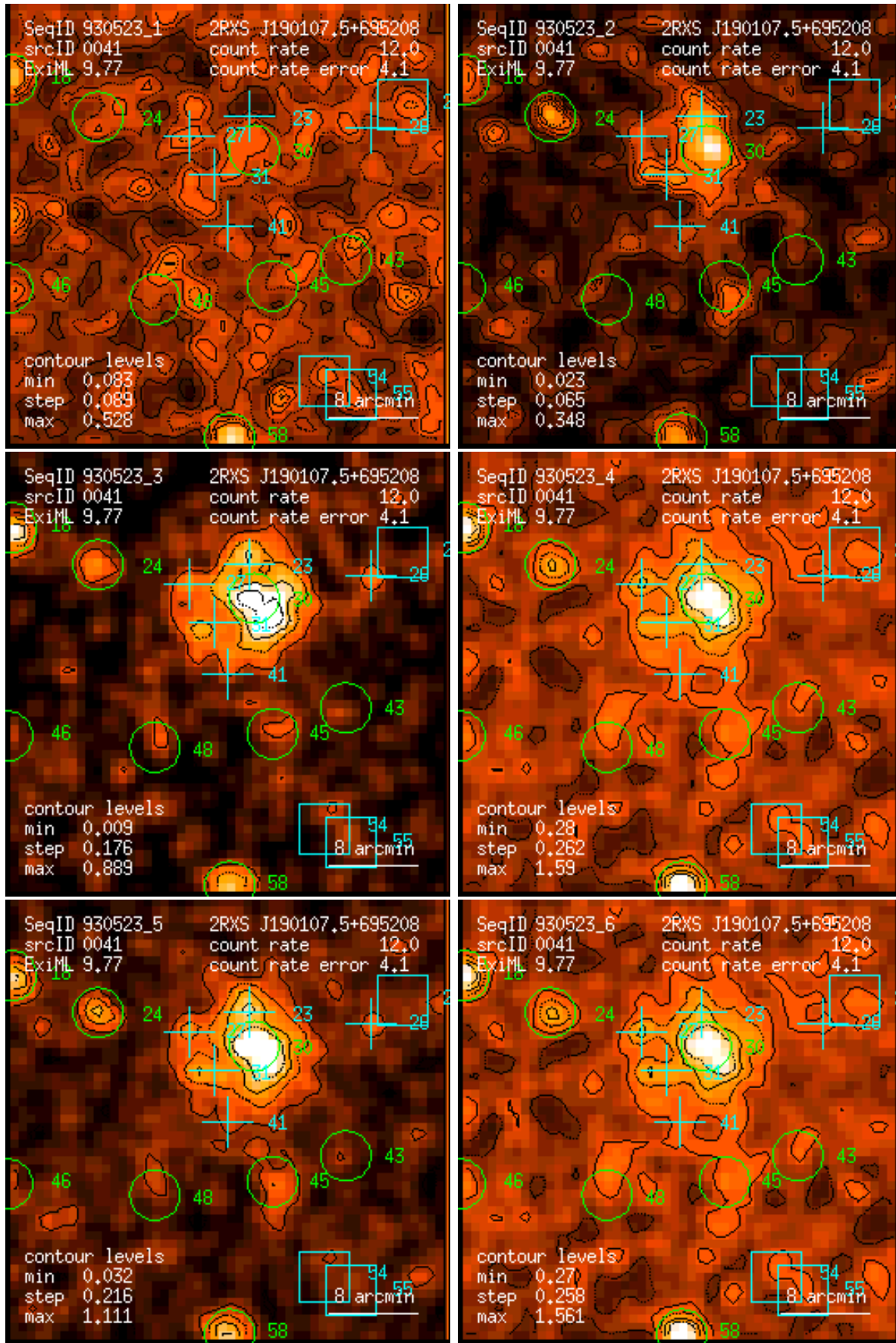
Figure 41: RASS 930523: detection 0041: band rate images, Gaussian filter: (1) PSPC channels 11 – 41, (2) 52 – 90, (3) 91 – 201, (4) 11 – 235, (5) 52 – 201, (6) 11 – 201. Broad band rates in counts/ks. Band rate contour levels in counts/ks/arcmin 2 .
