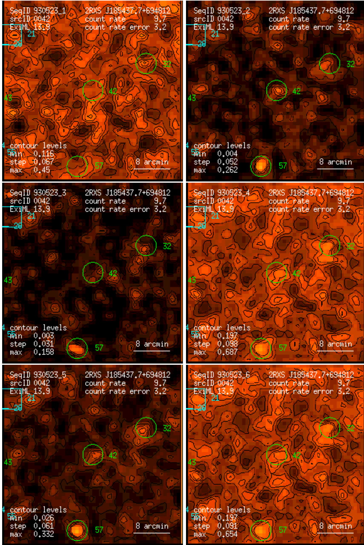
Figure 42: RASS 930523: detection 0042: band rate images, Gaussian filter: (1) PSPC channels 11 – 41, (2) 52 – 90, (3) 91 – 201, (4) 11 – 235, (5) 52 – 201, (6) 11 – 201. Broad band rates in counts/ks. Band rate contour levels in counts/ks/arcmin 2 .
