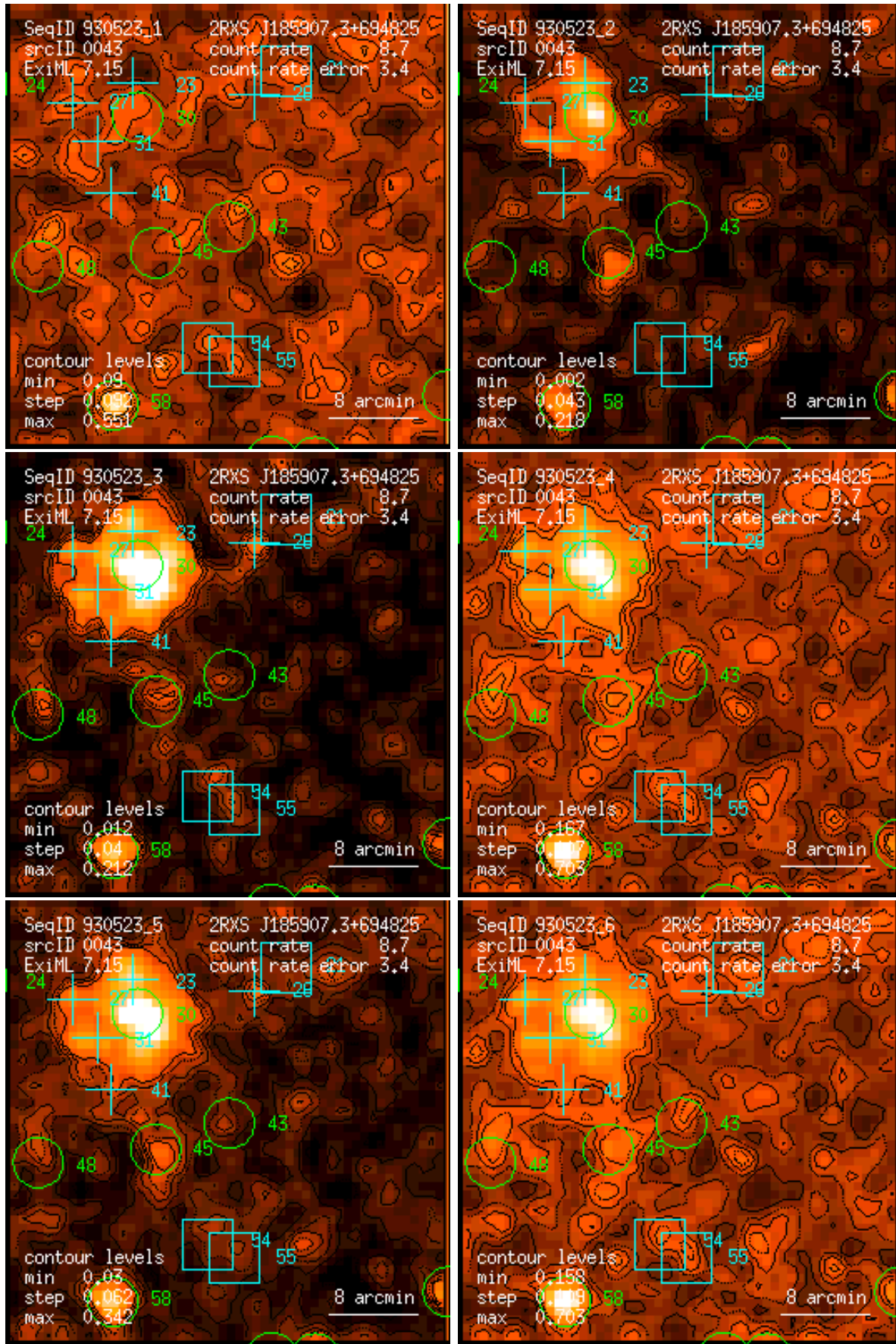
Figure 43: RASS 930523: detection 0043: band rate images, Gaussian filter: (1) PSPC channels 11 – 41, (2) 52 – 90, (3) 91 – 201, (4) 11 – 235, (5) 52 – 201, (6) 11 – 201. Broad band rates in counts/ks. Band rate contour levels in counts/ks/arcmin 2 .
