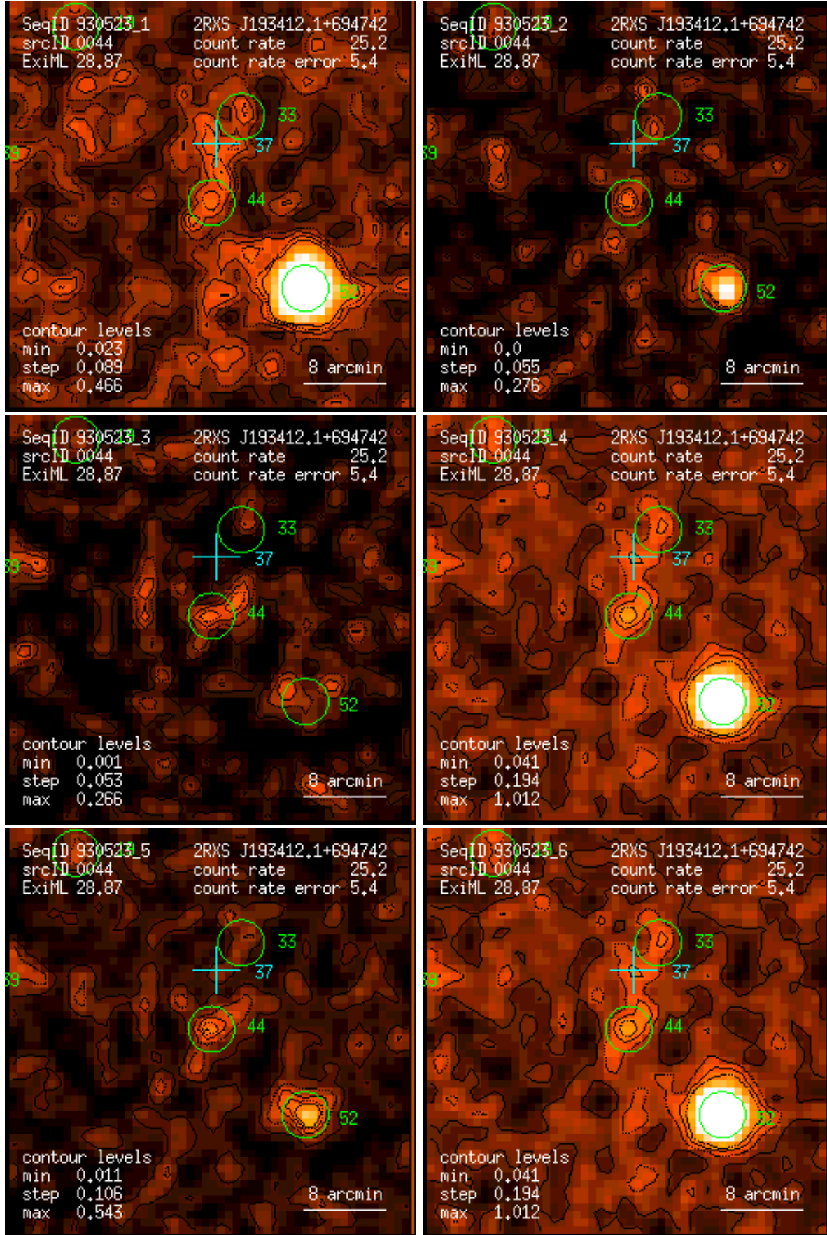
Figure 44: RASS 930523: detection 0044: band rate images, Gaussian filter: (1) PSPC channels 11 – 41, (2) 52 – 90, (3) 91 – 201, (4) 11 – 235, (5) 52 – 201, (6) 11 – 201. Broad band rates in counts/ks. Band rate contour levels in counts/ks/arcmin 2 .
