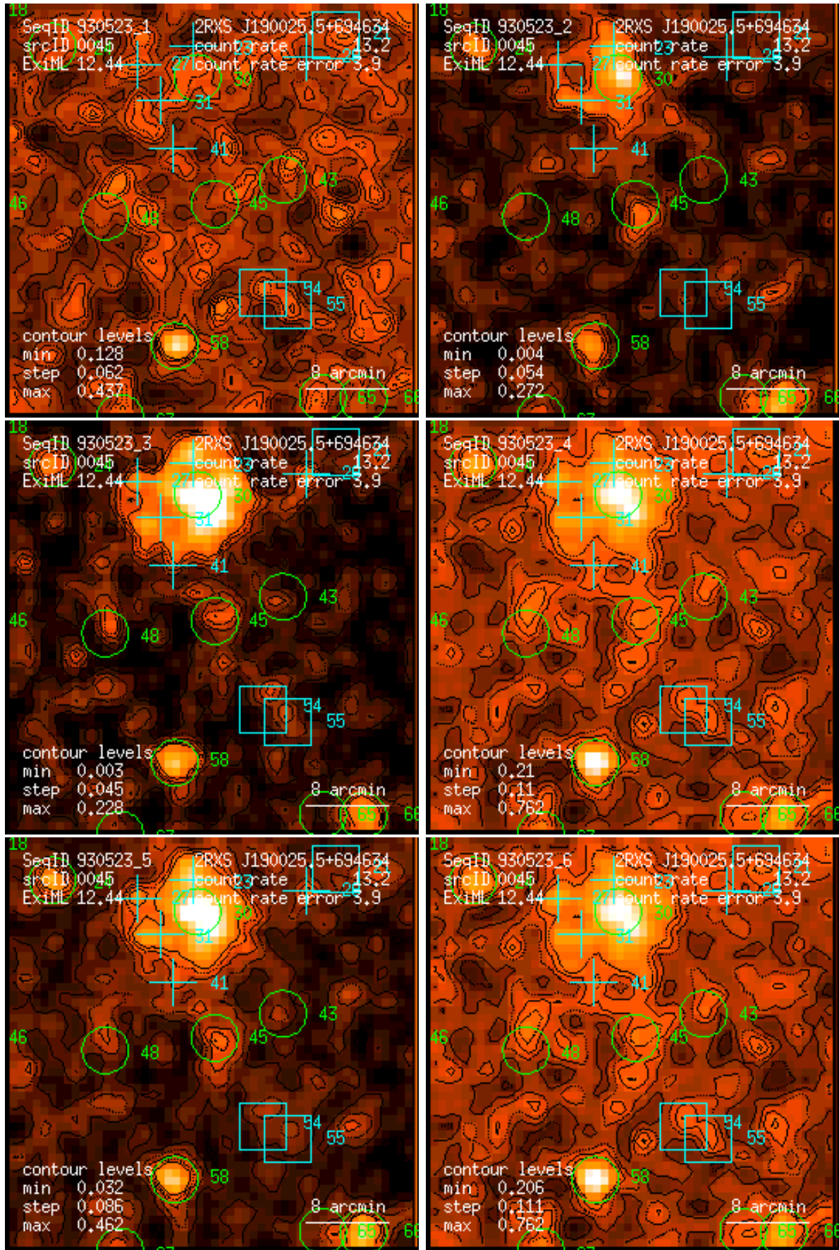
Figure 45: RASS 930523: detection 0045: band rate images, Gaussian filter: (1) PSPC channels 11 – 41, (2) 52 – 90, (3) 91 – 201, (4) 11 – 235, (5) 52 – 201, (6) 11 – 201. Broad band rates in counts/ks. Band rate contour levels in counts/ks/arcmin 2 .
