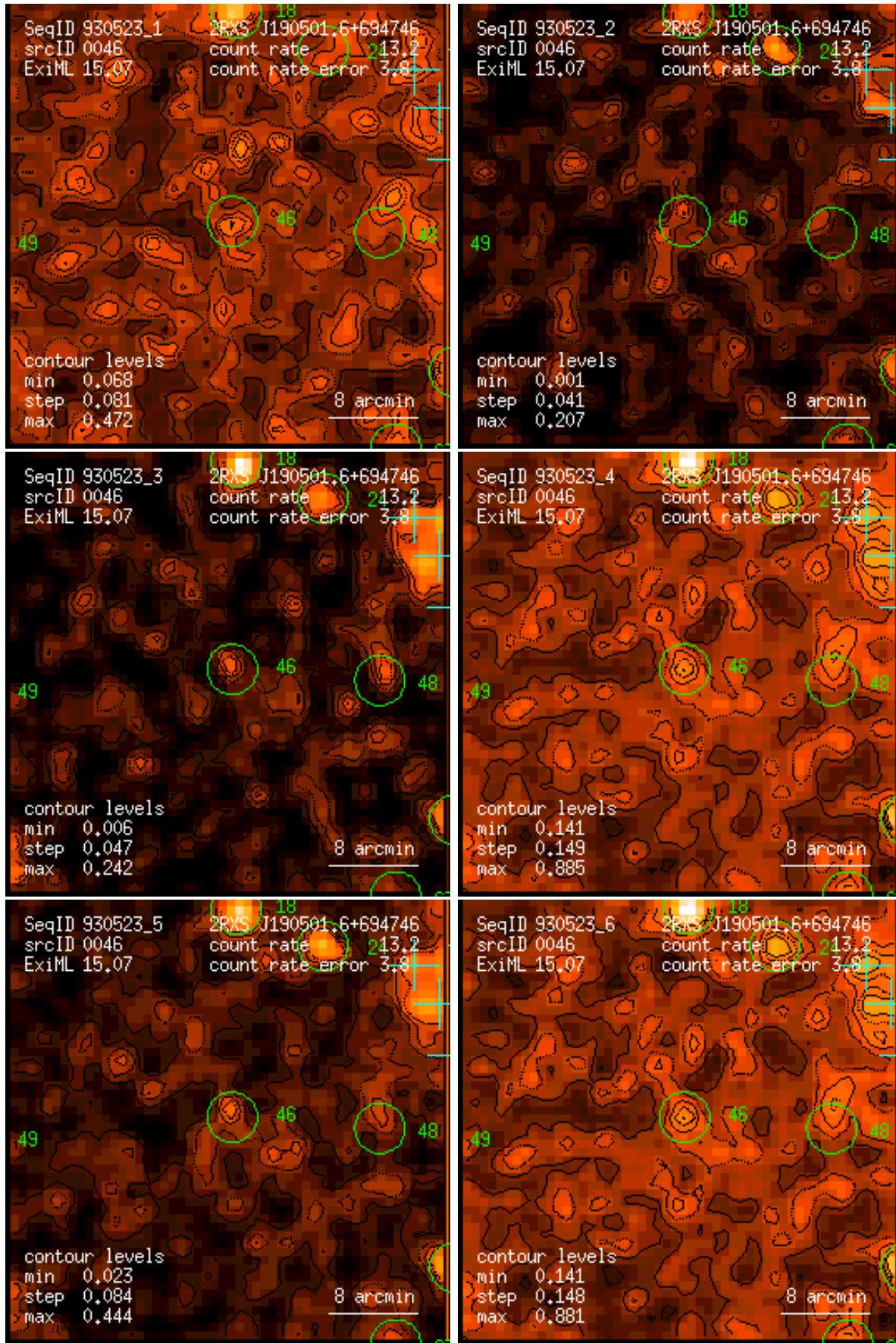
Figure 46: RASS 930523: detection 0046: band rate images, Gaussian filter: (1) PSPC channels 11 – 41, (2) 52 – 90, (3) 91 – 201, (4) 11 – 235, (5) 52 – 201, (6) 11 – 201. Broad band rates in counts/ks. Band rate contour levels in counts/ks/arcmin 2 .
