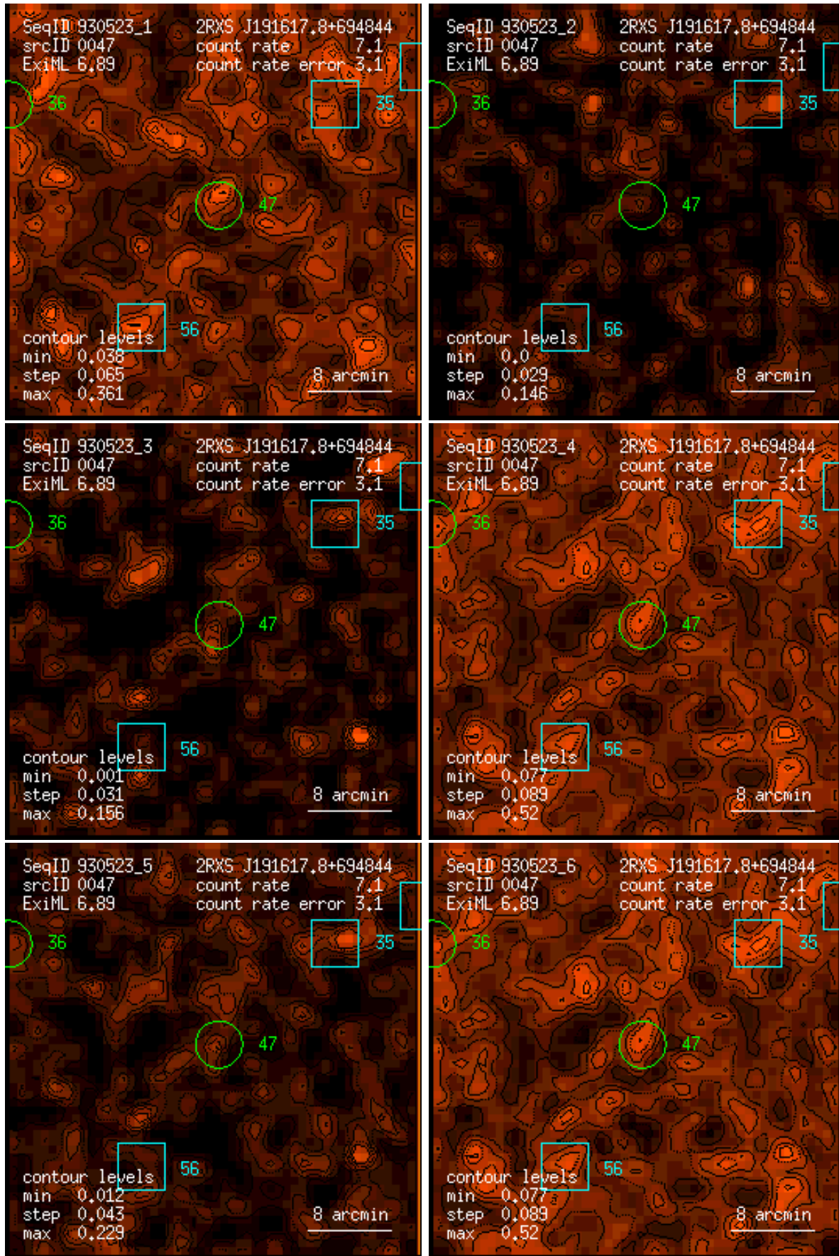
Figure 47: RASS 930523: detection 0047: band rate images, Gaussian filter: (1) PSPC channels 11 – 41, (2) 52 – 90, (3) 91 – 201, (4) 11 – 235, (5) 52 – 201, (6) 11 – 201. Broad band rates in counts/ks. Band rate contour levels in counts/ks/arcmin 2 .
