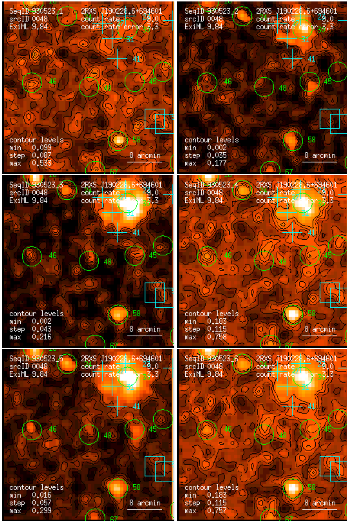
Figure 48: RASS 930523: detection 0048: band rate images, Gaussian filter: (1) PSPC channels 11 – 41, (2) 52 – 90, (3) 91 – 201, (4) 11 – 235, (5) 52 – 201, (6) 11 – 201. Broad band rates in counts/ks. Band rate contour levels in counts/ks/arcmin 2 .
