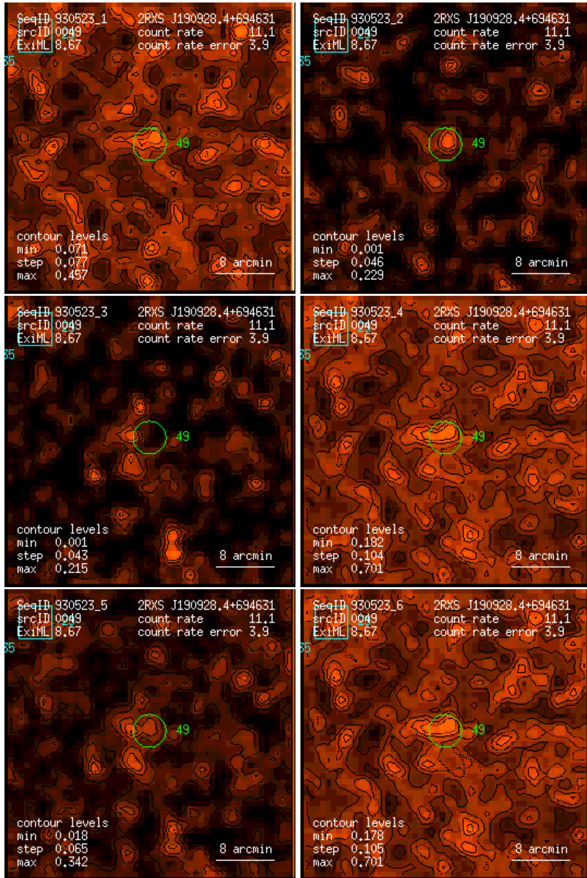
Figure 49: RASS 930523: detection 0049: band rate images, Gaussian filter: (1) PSPC channels 11 – 41, (2) 52 – 90, (3) 91 – 201, (4) 11 – 235, (5) 52 – 201, (6) 11 – 201. Broad band rates in counts/ks. Band rate contour levels in counts/ks/arcmin 2 .
