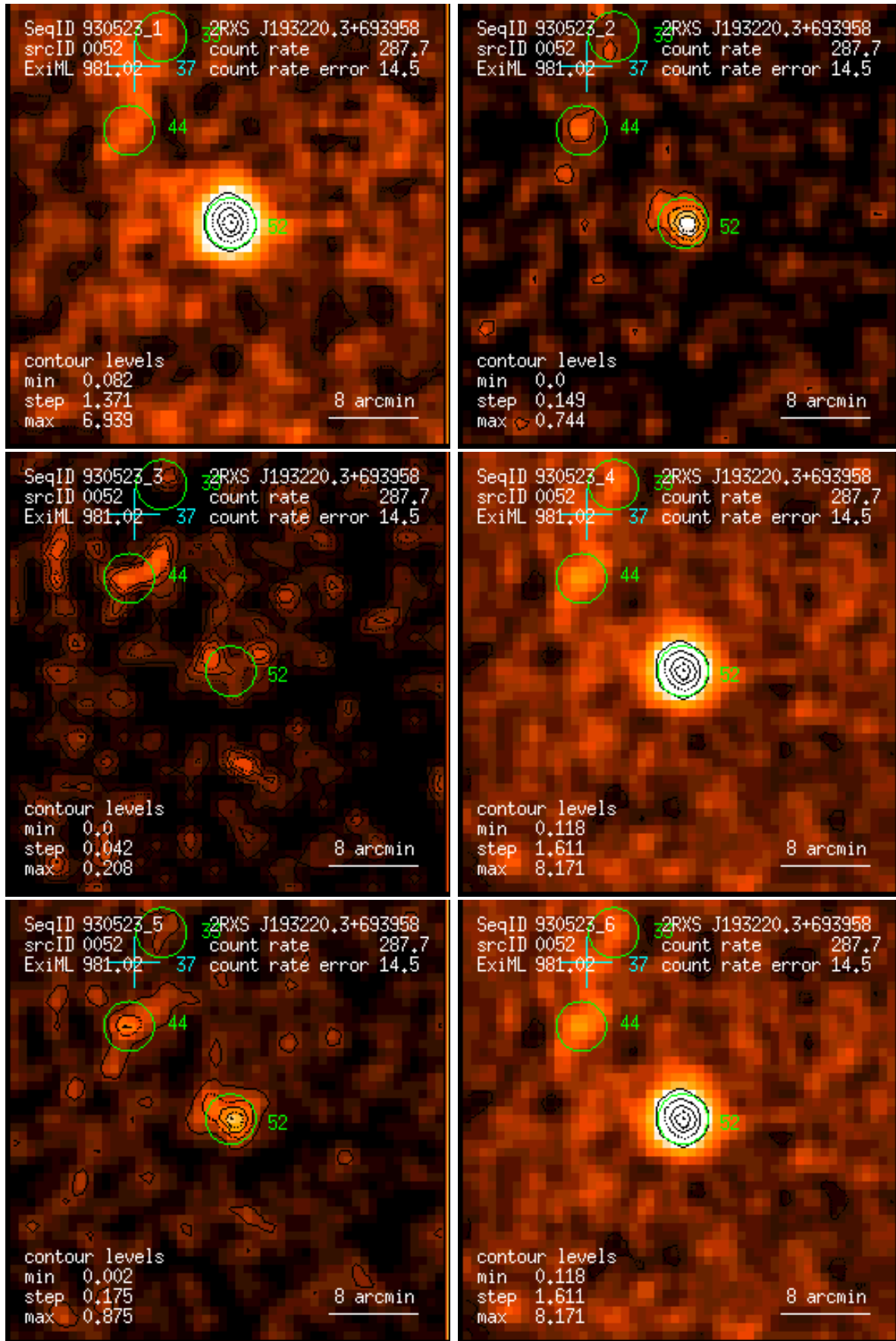
Figure 52: RASS 930523: detection 0052: band rate images, Gaussian filter: (1) PSPC channels 11 – 41, (2) 52 – 90, (3) 91 – 201, (4) 11 – 235, (5) 52 – 201, (6) 11 – 201. Broad band rates in counts/ks. Band rate contour levels in counts/ks/arcmin 2 .
