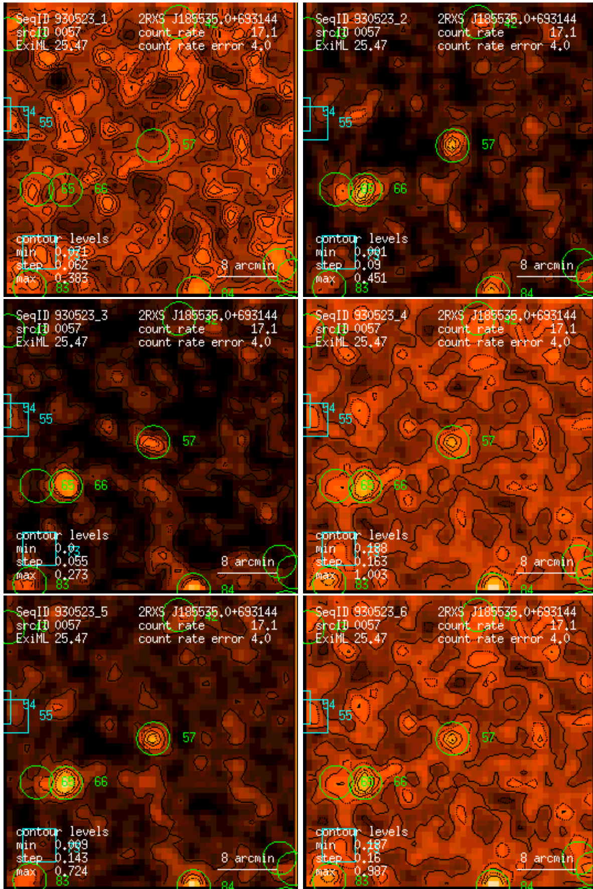
Figure 57: RASS 930523: detection 0057: band rate images, Gaussian filter: (1) PSPC channels 11 – 41, (2) 52 – 90, (3) 91 – 201, (4) 11 – 235, (5) 52 – 201, (6) 11 – 201. Broad band rates in counts/ks. Band rate contour levels in counts/ks/arcmin 2 .
