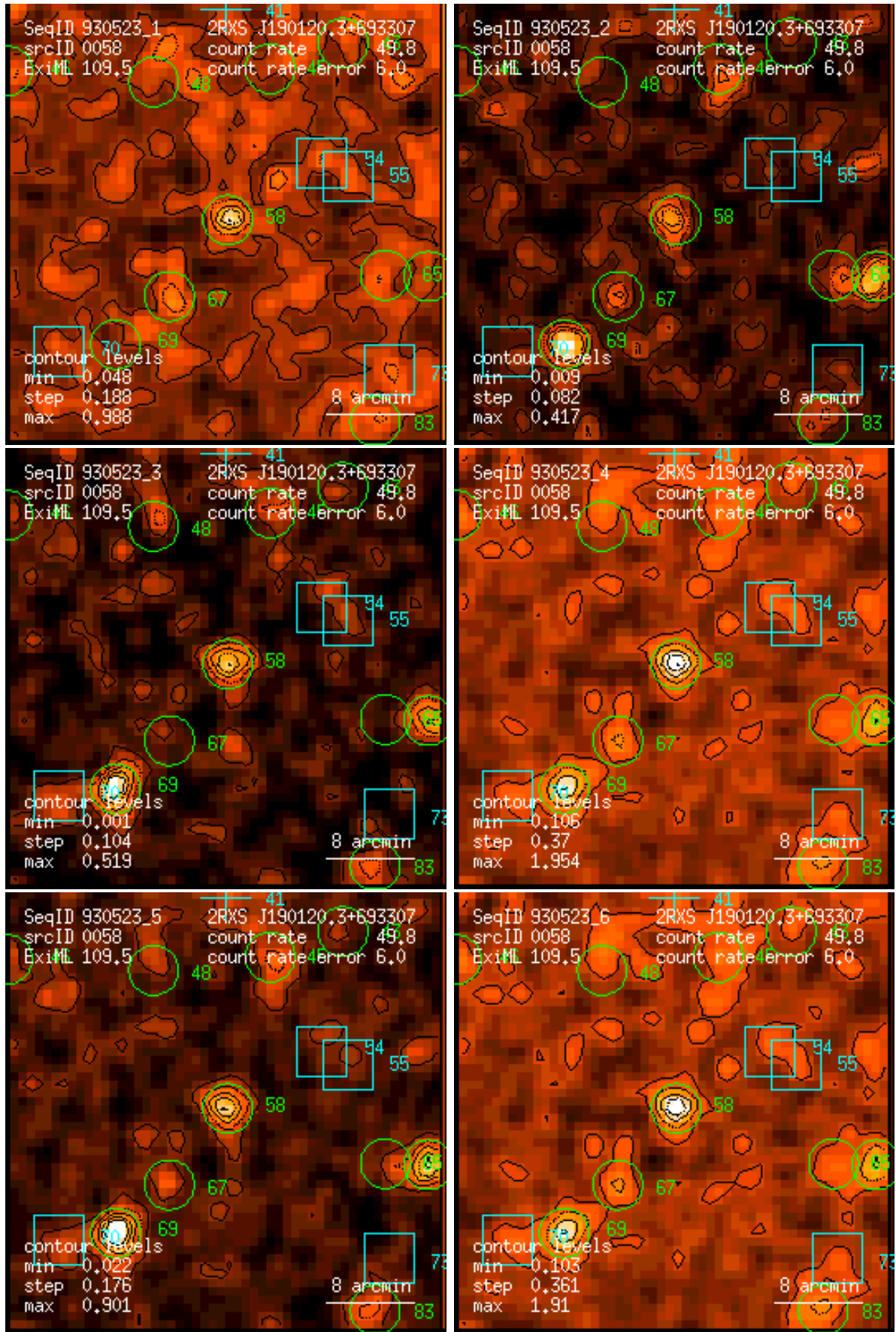
Figure 58: RASS 930523: detection 0058: band rate images, Gaussian filter: (1) PSPC channels 11 – 41, (2) 52 – 90, (3) 91 – 201, (4) 11 – 235, (5) 52 – 201, (6) 11 – 201. Broad band rates in counts/ks. Band rate contour levels in counts/ks/arcmin 2 .
