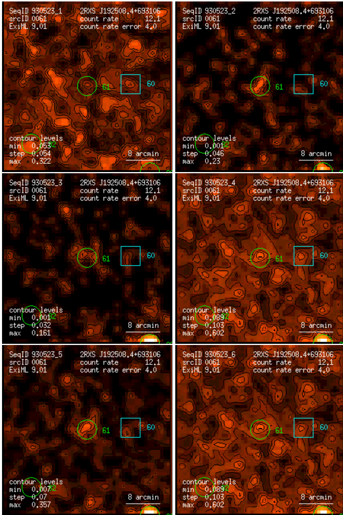
Figure 61: RASS 930523: detection 0061: band rate images, Gaussian filter: (1) PSPC channels 11 – 41, (2) 52 – 90, (3) 91 – 201, (4) 11 – 235, (5) 52 – 201, (6) 11 – 201. Broad band rates in counts/ks. Band rate contour levels in counts/ks/arcmin 2 .
