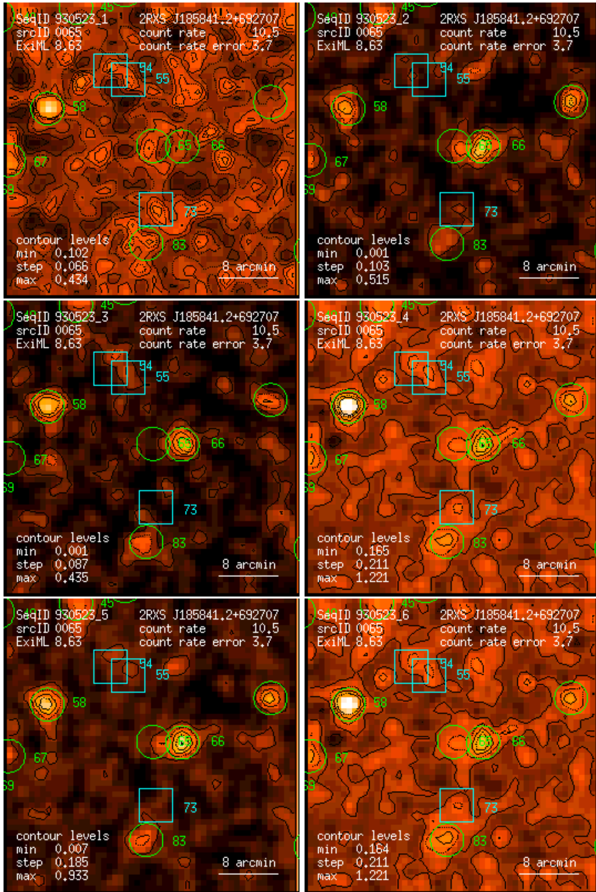
Figure 65: RASS 930523: detection 0065: band rate images, Gaussian filter: (1) PSPC channels 11 – 41, (2) 52 – 90, (3) 91 – 201, (4) 11 – 235, (5) 52 – 201, (6) 11 – 201. Broad band rates in counts/ks. Band rate contour levels in counts/ks/arcmin 2 .
