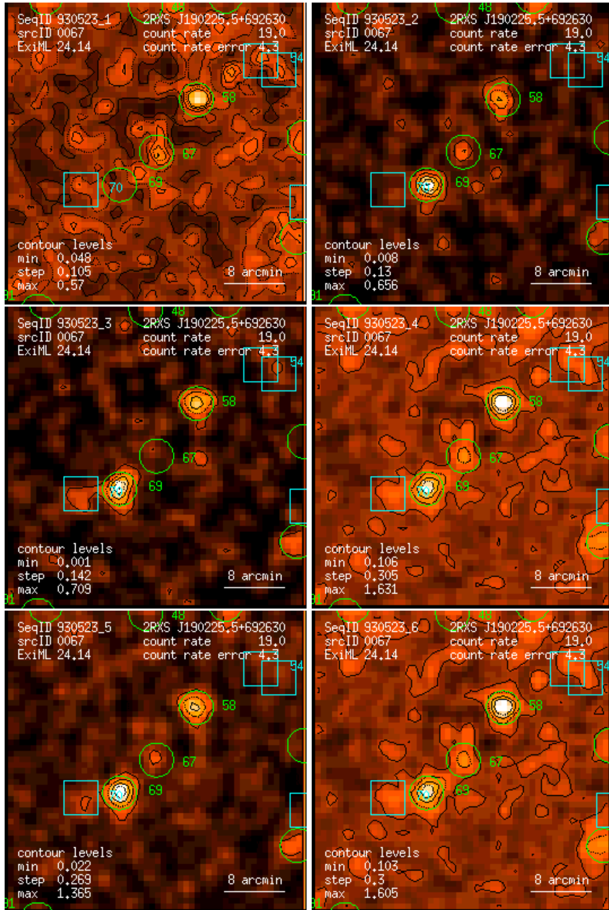
Figure 67: RASS 930523: detection 0067: band rate images, Gaussian filter: (1) PSPC channels 11 – 41, (2) 52 – 90, (3) 91 – 201, (4) 11 – 235, (5) 52 – 201, (6) 11 – 201. Broad band rates in counts/ks. Band rate contour levels in counts/ks/arcmin 2 .
